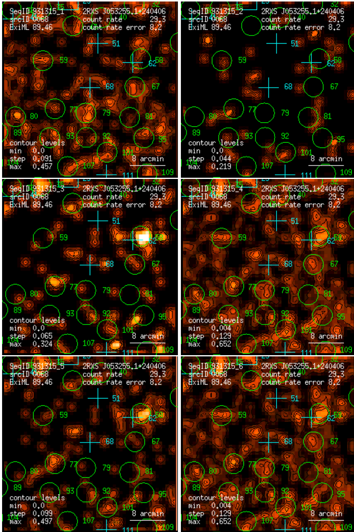
Figure 68: RASS 931315: detection 0068: band rate images, Gaussian filter: (1) PSPC channels 11 – 41, (2) 52 – 90, (3) 91 – 201, (4) 11 – 235, (5) 52 – 201, (6) 11 – 201. Broad band rates in counts/ks. Band rate contour levels in counts/ks/arcmin 2 .
