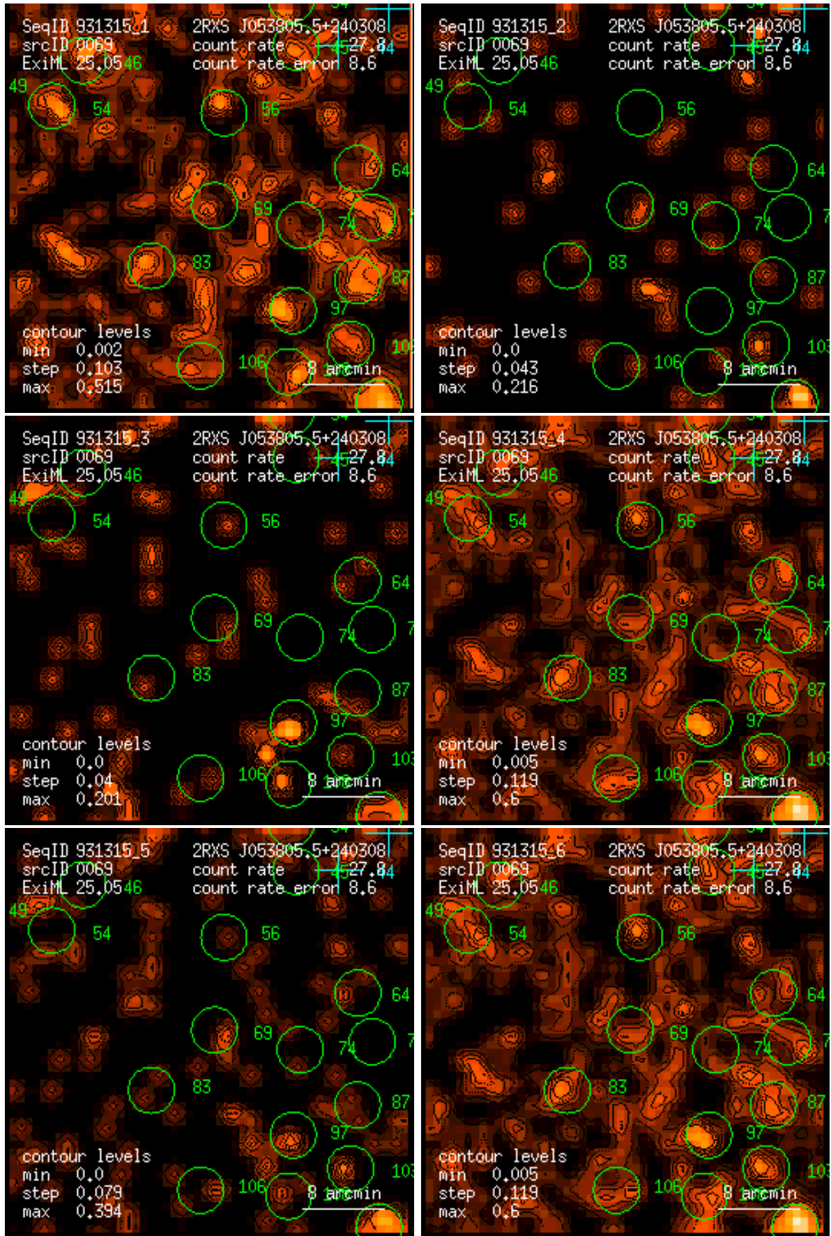
Figure 69: RASS 931315: detection 0069: band rate images, Gaussian filter: (1) PSPC channels 11 – 41, (2) 52 – 90, (3) 91 – 201, (4) 11 – 235, (5) 52 – 201, (6) 11 – 201. Broad band rates in counts/ks. Band rate contour levels in counts/ks/arcmin 2 .
