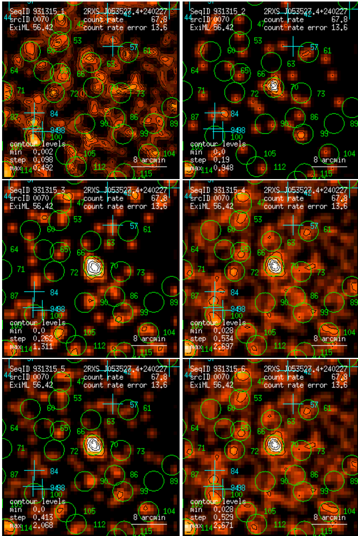
Figure 70: RASS 931315: detection 0070: band rate images, Gaussian filter: (1) PSPC channels 11 – 41, (2) 52 – 90, (3) 91 – 201, (4) 11 – 235, (5) 52 – 201, (6) 11 – 201. Broad band rates in counts/ks. Band rate contour levels in counts/ks/arcmin 2 .
