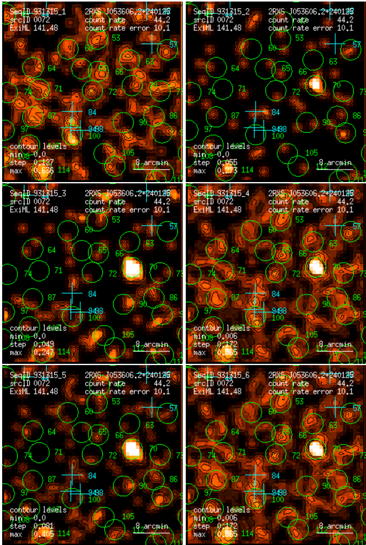
Figure 72: RASS 931315: detection 0072: band rate images, Gaussian filter: (1) PSPC channels 11 – 41, (2) 52 – 90, (3) 91 – 201, (4) 11 – 235, (5) 52 – 201, (6) 11 – 201. Broad band rates in counts/ks. Band rate contour levels in counts/ks/arcmin 2 .
