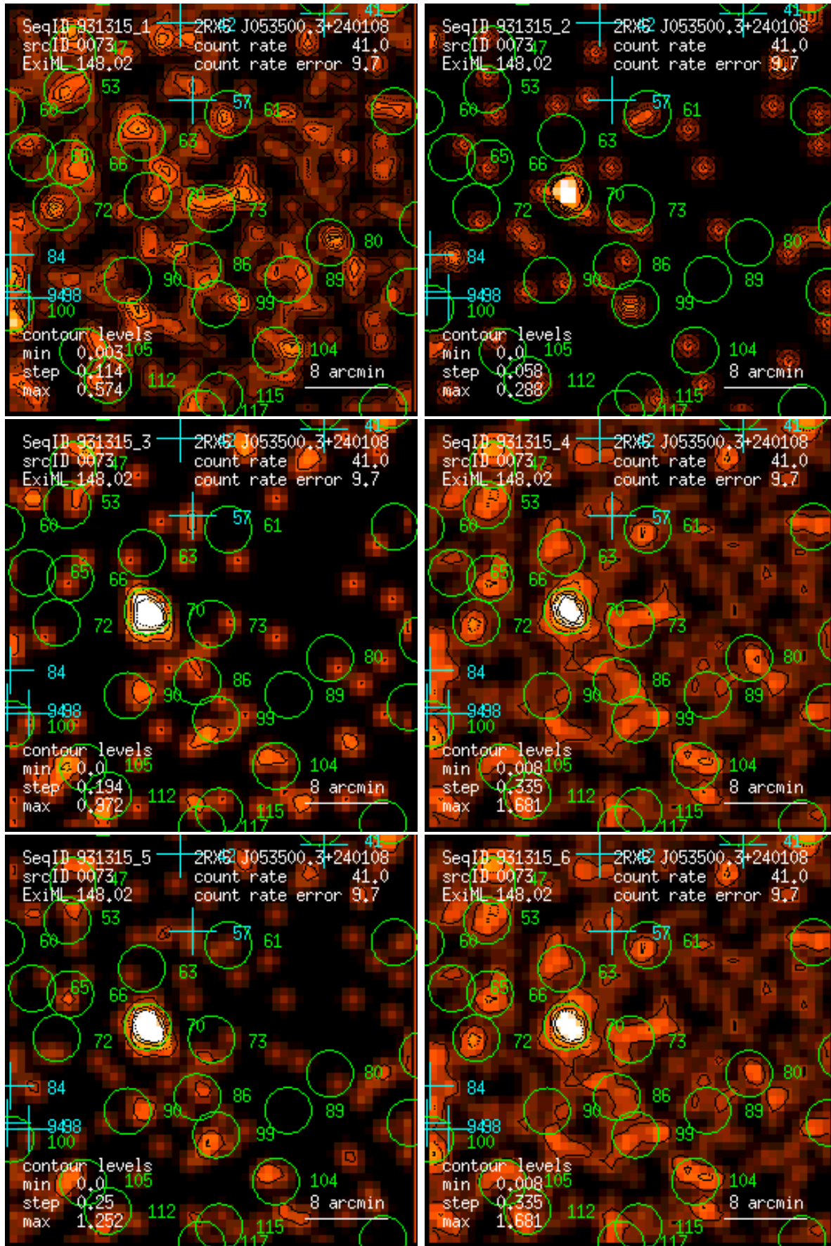
Figure 73: RASS 931315: detection 0073: band rate images, Gaussian filter: (1) PSPC channels 11 – 41, (2) 52 – 90, (3) 91 – 201, (4) 11 – 235, (5) 52 – 201, (6) 11 – 201. Broad band rates in counts/ks. Band rate contour levels in counts/ks/arcmin 2 .
