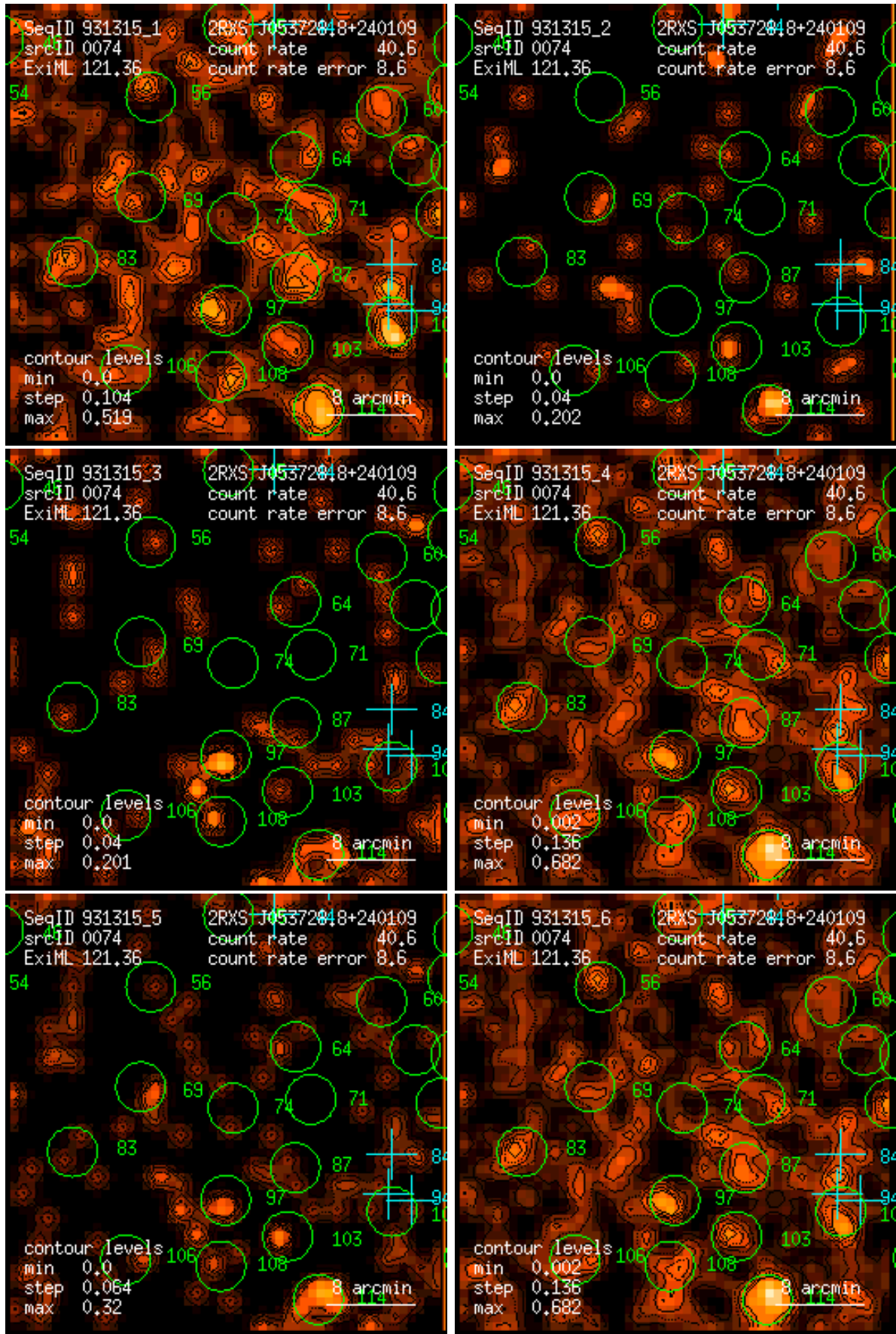
Figure 74: RASS 931315: detection 0074: band rate images, Gaussian filter: (1) PSPC channels 11 – 41, (2) 52 – 90, (3) 91 – 201, (4) 11 – 235, (5) 52 – 201, (6) 11 – 201. Broad band rates in counts/ks. Band rate contour levels in counts/ks/arcmin 2 .
