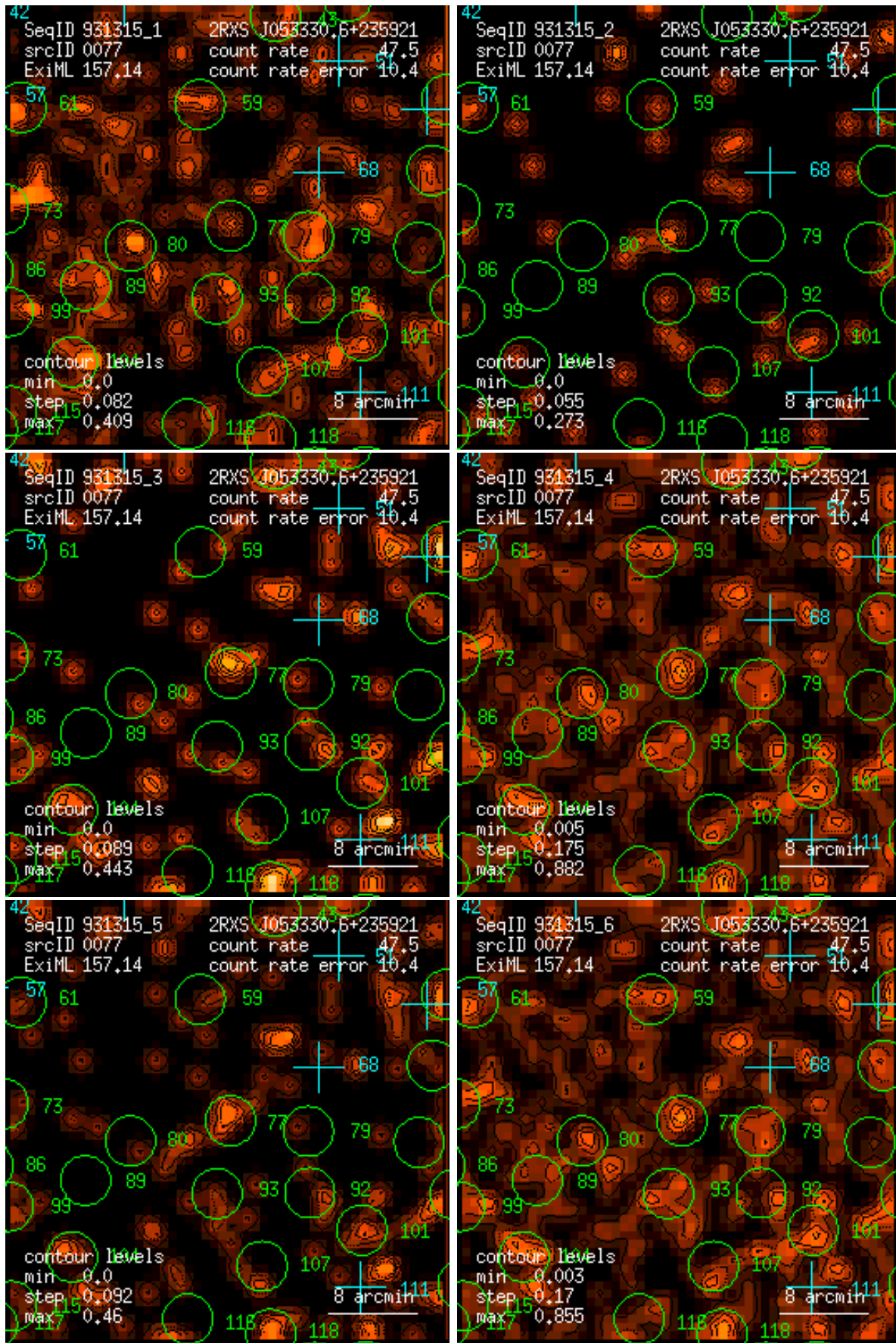
Figure 77: RASS 931315: detection 0077: band rate images, Gaussian filter: (1) PSPC channels 11 – 41, (2) 52 – 90, (3) 91 – 201, (4) 11 – 235, (5) 52 – 201, (6) 11 – 201. Broad band rates in counts/ks. Band rate contour levels in counts/ks/arcmin 2 .
