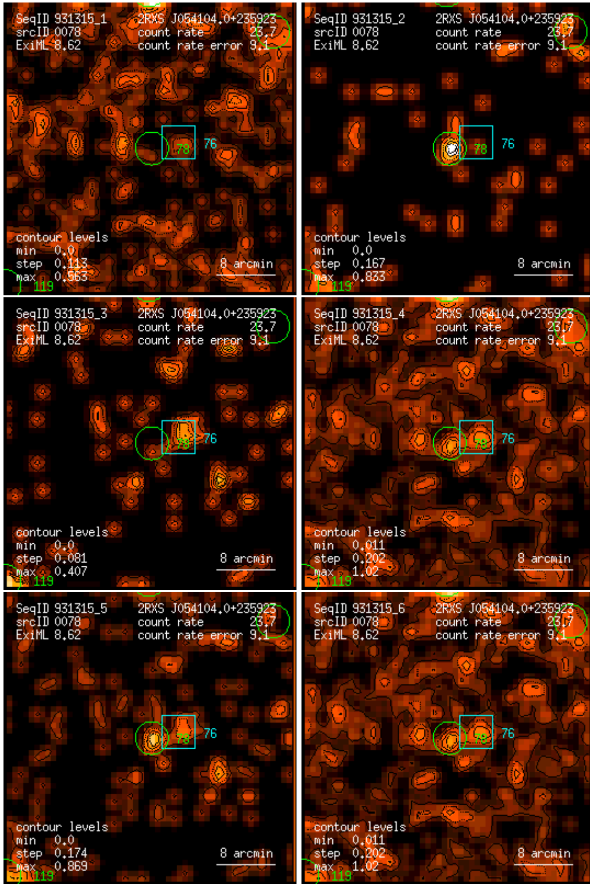
Figure 78: RASS 931315: detection 0078: band rate images, Gaussian filter: (1) PSPC channels 11 – 41, (2) 52 – 90, (3) 91 – 201, (4) 11 – 235, (5) 52 – 201, (6) 11 – 201. Broad band rates in counts/ks. Band rate contour levels in counts/ks/arcmin 2 .
