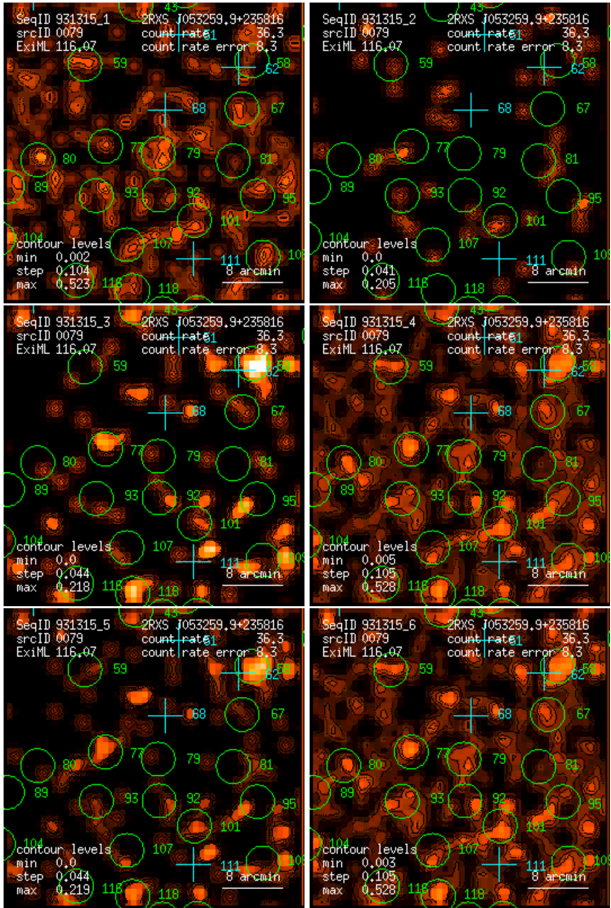
Figure 79: RASS 931315: detection 0079: band rate images, Gaussian filter: (1) PSPC channels 11 – 41, (2) 52 – 90, (3) 91 – 201, (4) 11 – 235, (5) 52 – 201, (6) 11 – 201. Broad band rates in counts/ks. Band rate contour levels in counts/ks/arcmin 2 .
