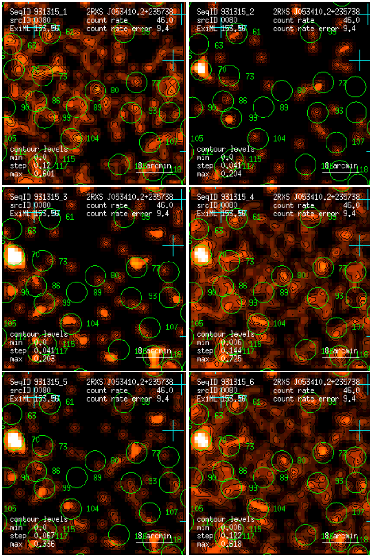
Figure 80: RASS 931315: detection 0080: band rate images, Gaussian filter: (1) PSPC channels 11 – 41, (2) 52 – 90, (3) 91 – 201, (4) 11 – 235, (5) 52 – 201, (6) 11 – 201. Broad band rates in counts/ks. Band rate contour levels in counts/ks/arcmin 2 .
