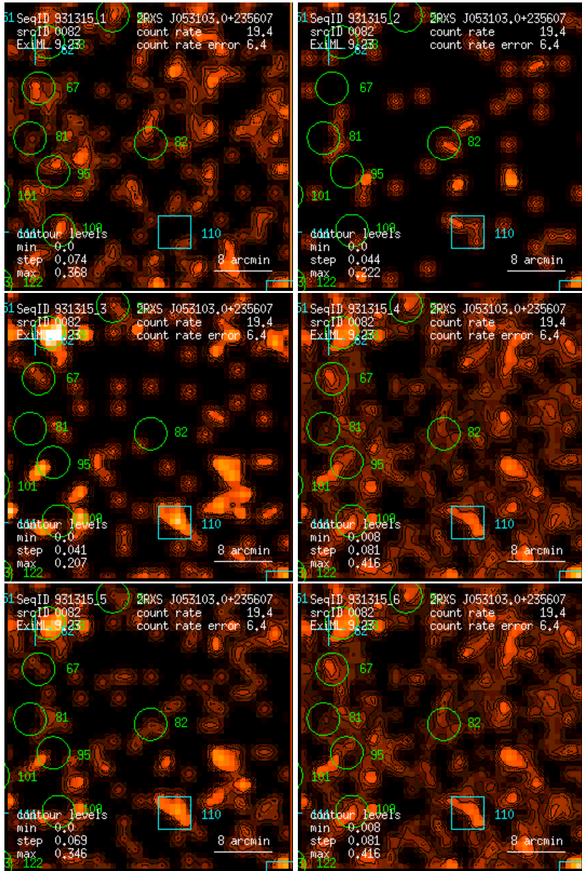
Figure 82: RASS 931315: detection 0082: band rate images, Gaussian filter: (1) PSPC channels 11 – 41, (2) 52 – 90, (3) 91 – 201, (4) 11 – 235, (5) 52 – 201, (6) 11 – 201. Broad band rates in counts/ks. Band rate contour levels in counts/ks/arcmin 2 .
