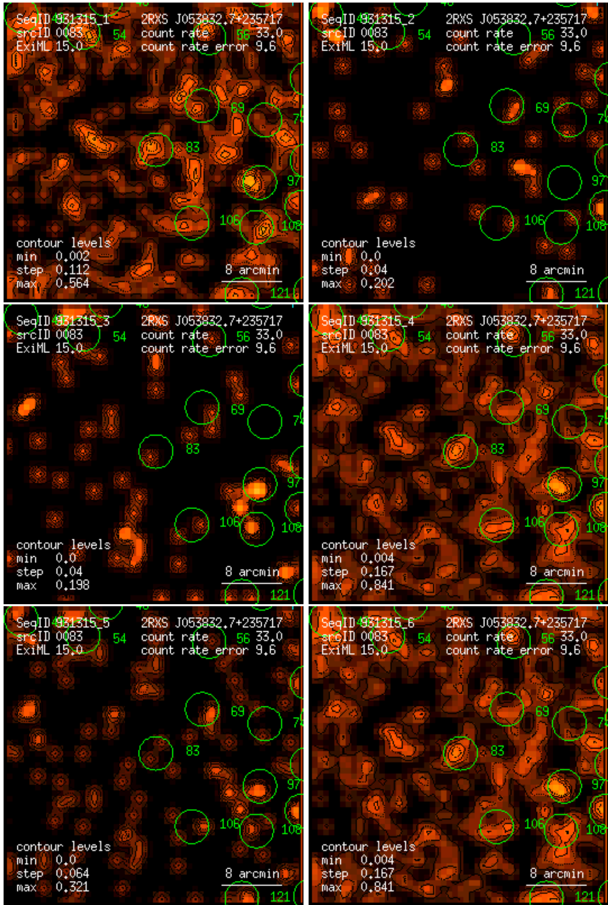
Figure 83: RASS 931315: detection 0083: band rate images, Gaussian filter: (1) PSPC channels 11 – 41, (2) 52 – 90, (3) 91 – 201, (4) 11 – 235, (5) 52 – 201, (6) 11 – 201. Broad band rates in counts/ks. Band rate contour levels in counts/ks/arcmin 2 .
