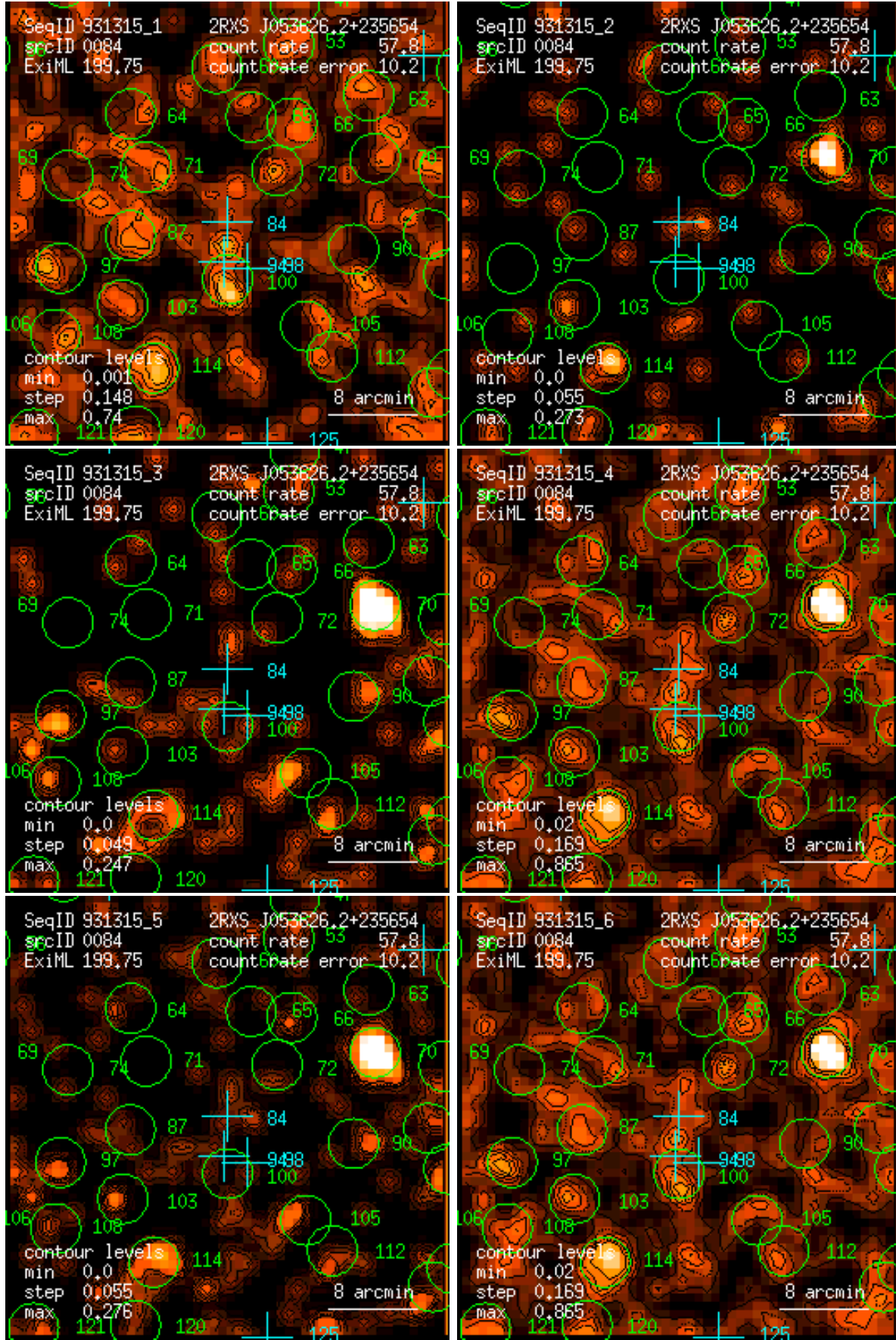
Figure 84: RASS 931315: detection 0084: band rate images, Gaussian filter: (1) PSPC channels 11 – 41, (2) 52 – 90, (3) 91 – 201, (4) 11 – 235, (5) 52 – 201, (6) 11 – 201. Broad band rates in counts/ks. Band rate contour levels in counts/ks/arcmin 2 .
