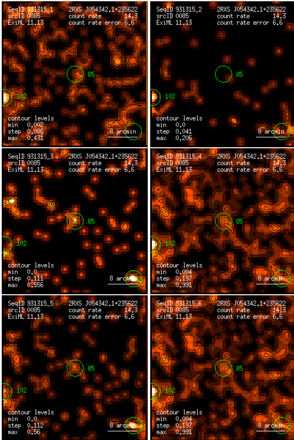
Figure 85: RASS 931315: detection 0085: band rate images, Gaussian filter: (1) PSPC channels 11 – 41, (2) 52 – 90, (3) 91 – 201, (4) 11 – 235, (5) 52 – 201, (6) 11 – 201. Broad band rates in counts/ks. Band rate contour levels in counts/ks/arcmin 2 .
