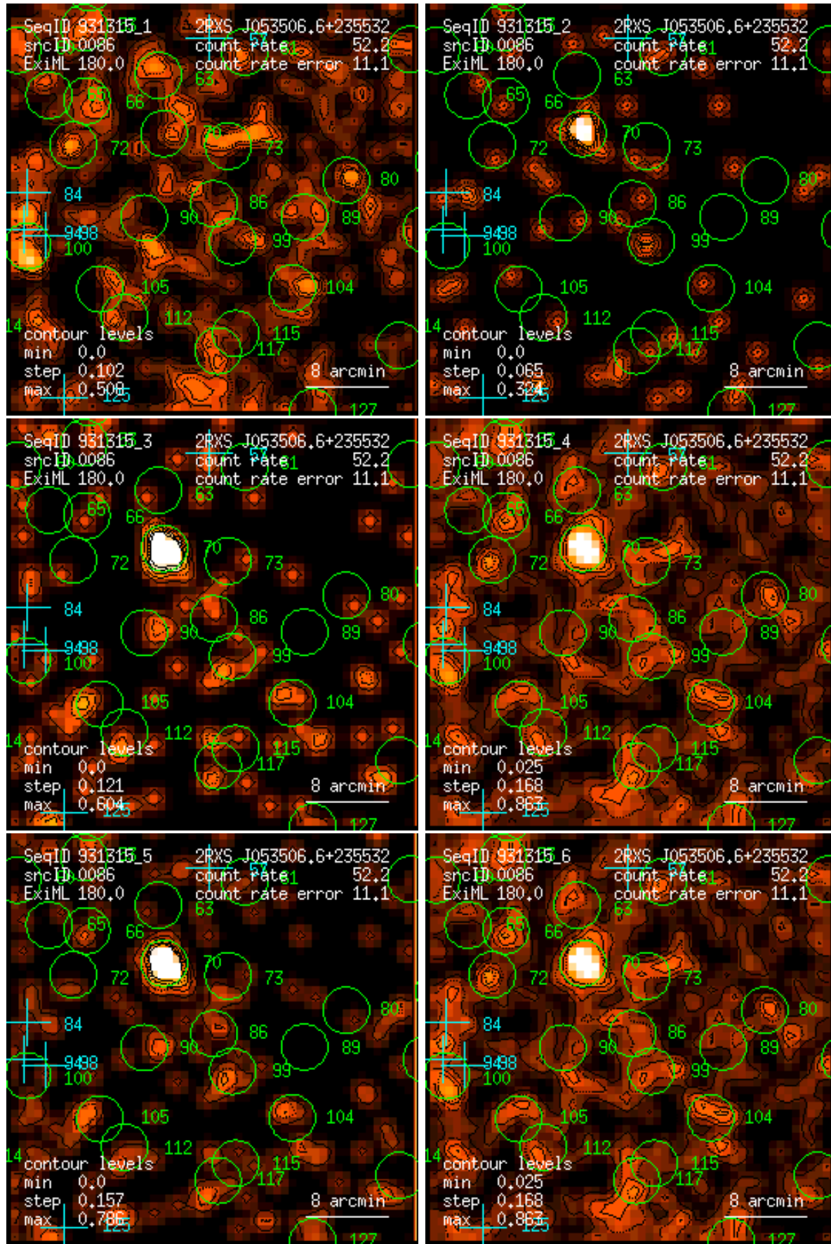
Figure 86: RASS 931315: detection 0086: band rate images, Gaussian filter: (1) PSPC channels 11 – 41, (2) 52 – 90, (3) 91 – 201, (4) 11 – 235, (5) 52 – 201, (6) 11 – 201. Broad band rates in counts/ks. Band rate contour levels in counts/ks/arcmin 2 .
