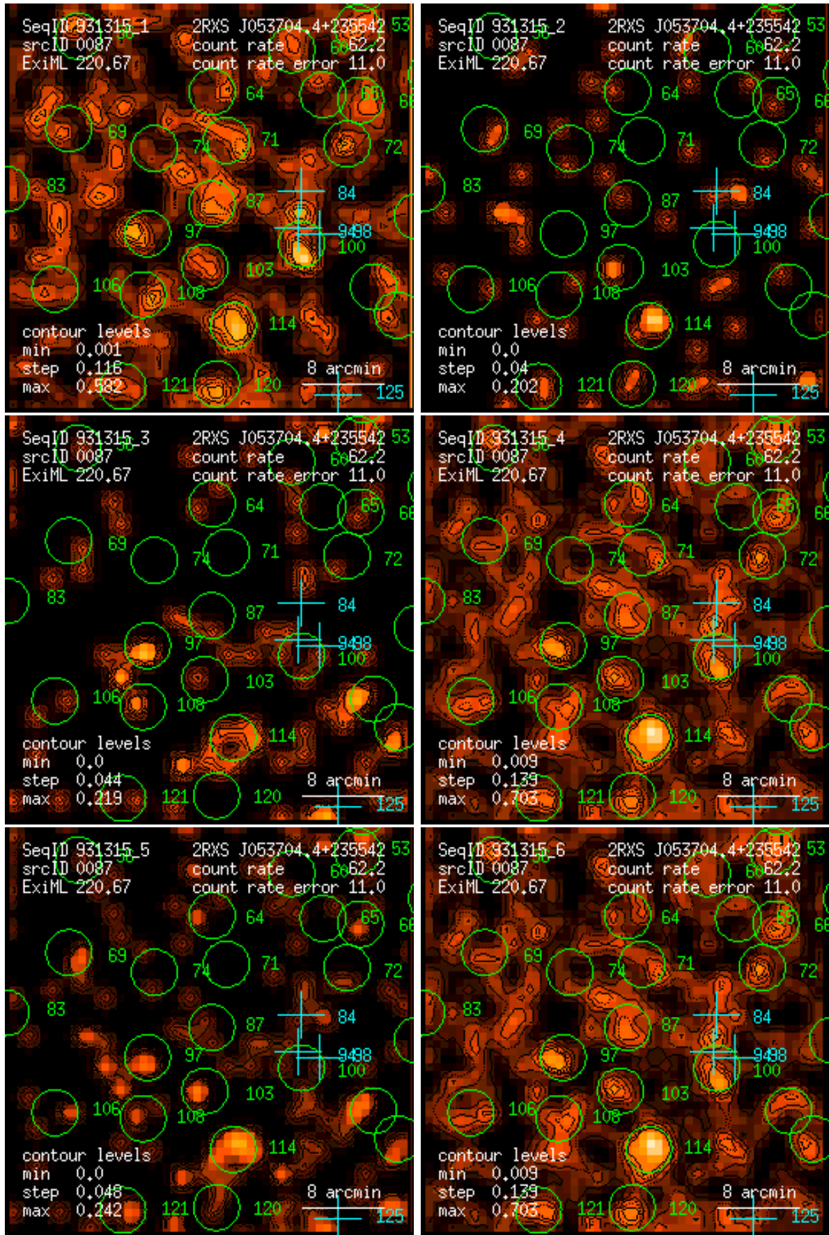
Figure 87: RASS 931315: detection 0087: band rate images, Gaussian filter: (1) PSPC channels 11 – 41, (2) 52 – 90, (3) 91 – 201, (4) 11 – 235, (5) 52 – 201, (6) 11 – 201. Broad band rates in counts/ks. Band rate contour levels in counts/ks/arcmin 2 .
