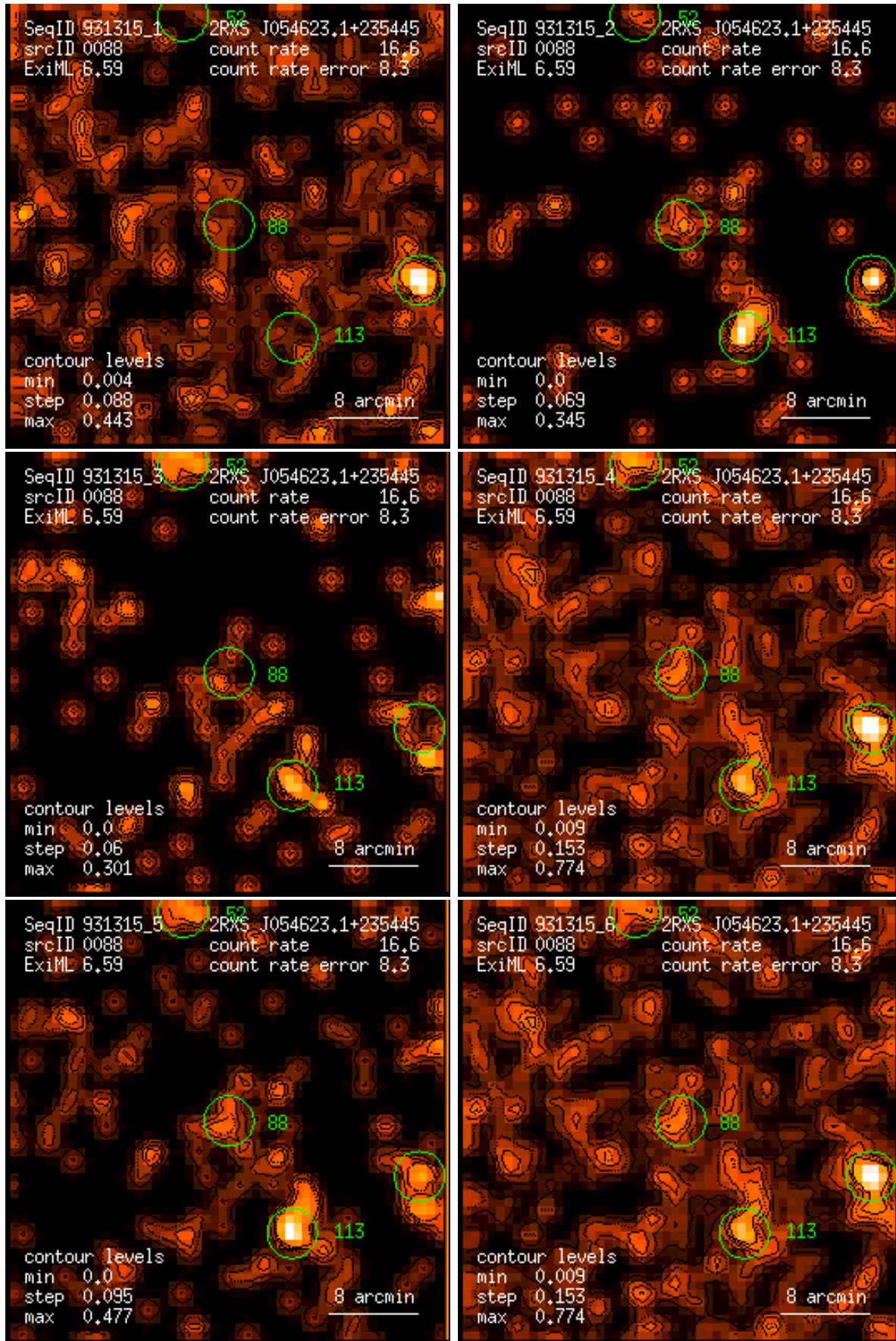
Figure 88: RASS 931315: detection 0088: band rate images, Gaussian filter: (1) PSPC channels 11 – 41, (2) 52 – 90, (3) 91 – 201, (4) 11 – 235, (5) 52 – 201, (6) 11 – 201. Broad band rates in counts/ks. Band rate contour levels in counts/ks/arcmin 2 .
