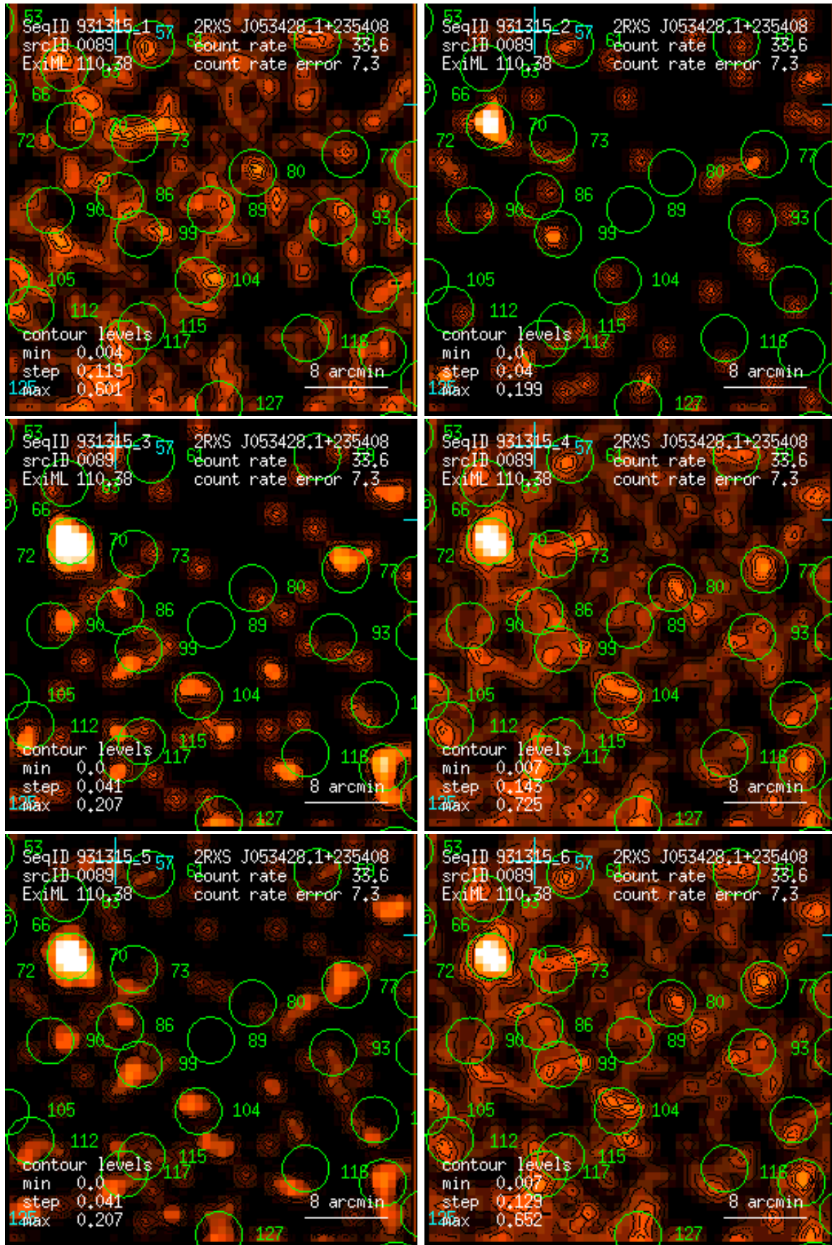
Figure 89: RASS 931315: detection 0089: band rate images, Gaussian filter: (1) PSPC channels 11 – 41, (2) 52 – 90, (3) 91 – 201, (4) 11 – 235, (5) 52 – 201, (6) 11 – 201. Broad band rates in counts/ks. Band rate contour levels in counts/ks/arcmin 2 .
