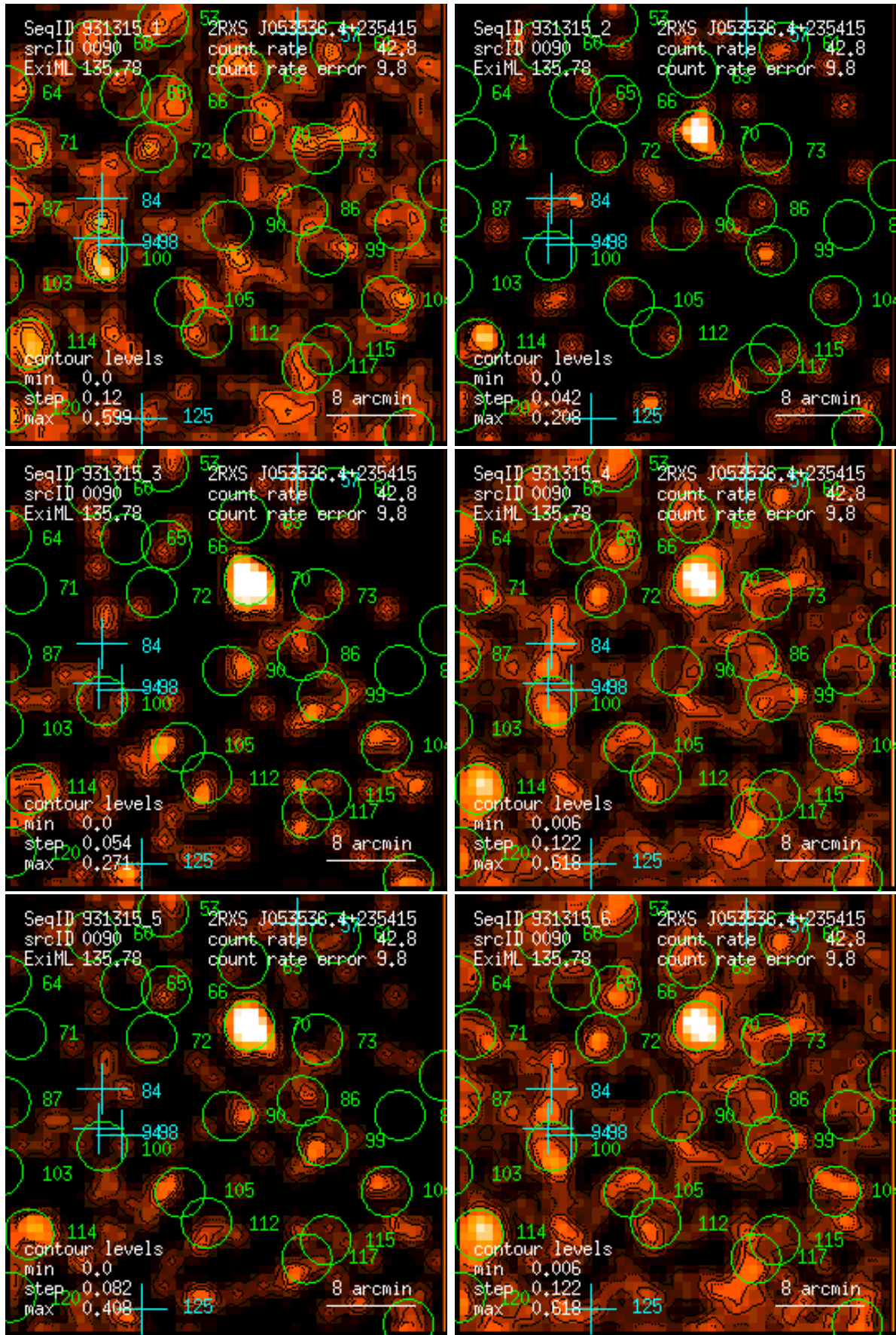
Figure 90: RASS 931315: detection 0090: band rate images, Gaussian filter: (1) PSPC channels 11 – 41, (2) 52 – 90, (3) 91 – 201, (4) 11 – 235, (5) 52 – 201, (6) 11 – 201. Broad band rates in counts/ks. Band rate contour levels in counts/ks/arcmin 2 .
