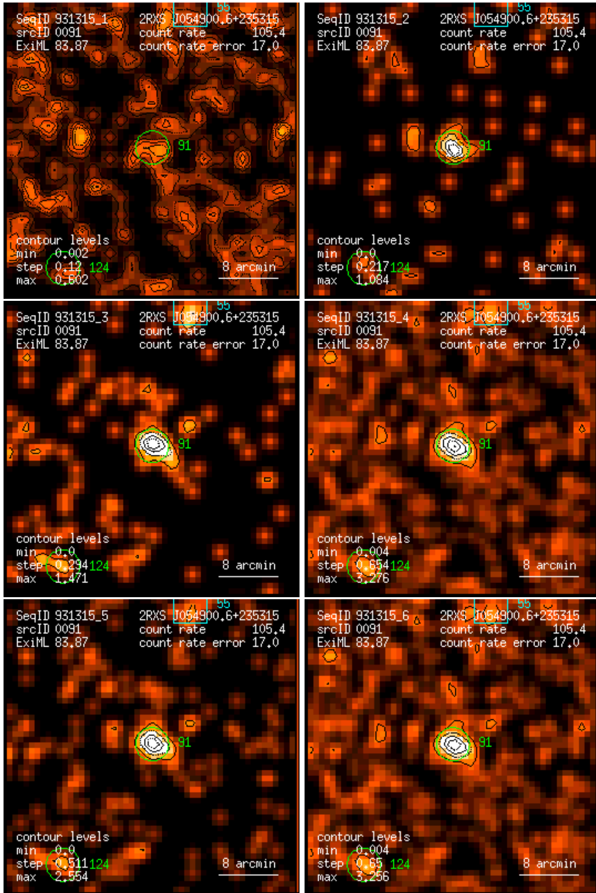
Figure 91: RASS 931315: detection 0091: band rate images, Gaussian filter: (1) PSPC channels 11 – 41, (2) 52 – 90, (3) 91 – 201, (4) 11 – 235, (5) 52 – 201, (6) 11 – 201. Broad band rates in counts/ks. Band rate contour levels in counts/ks/arcmin 2 .
