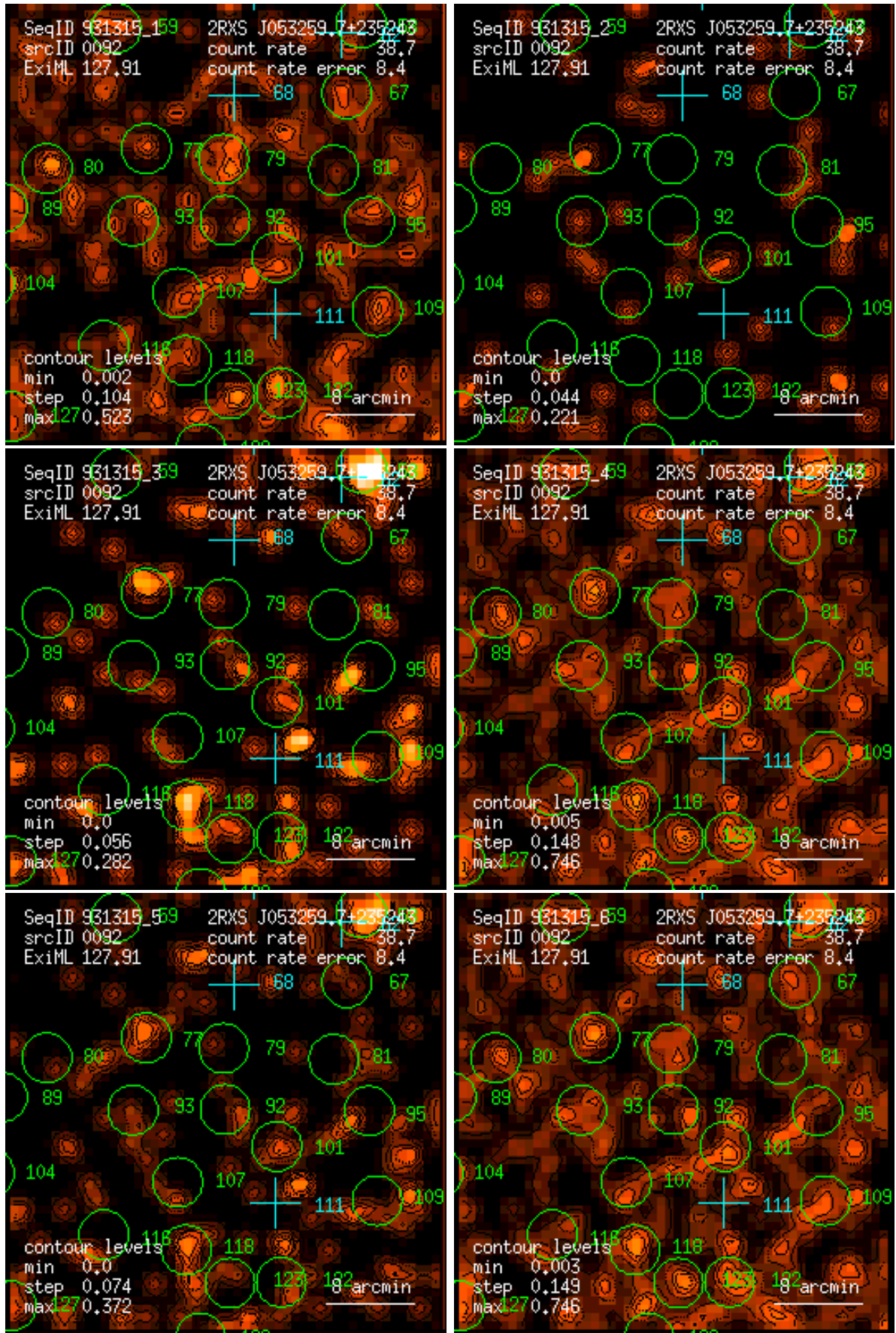
Figure 92: RASS 931315: detection 0092: band rate images, Gaussian filter: (1) PSPC channels 11 – 41, (2) 52 – 90, (3) 91 – 201, (4) 11 – 235, (5) 52 – 201, (6) 11 – 201. Broad band rates in counts/ks. Band rate contour levels in counts/ks/arcmin 2 .
