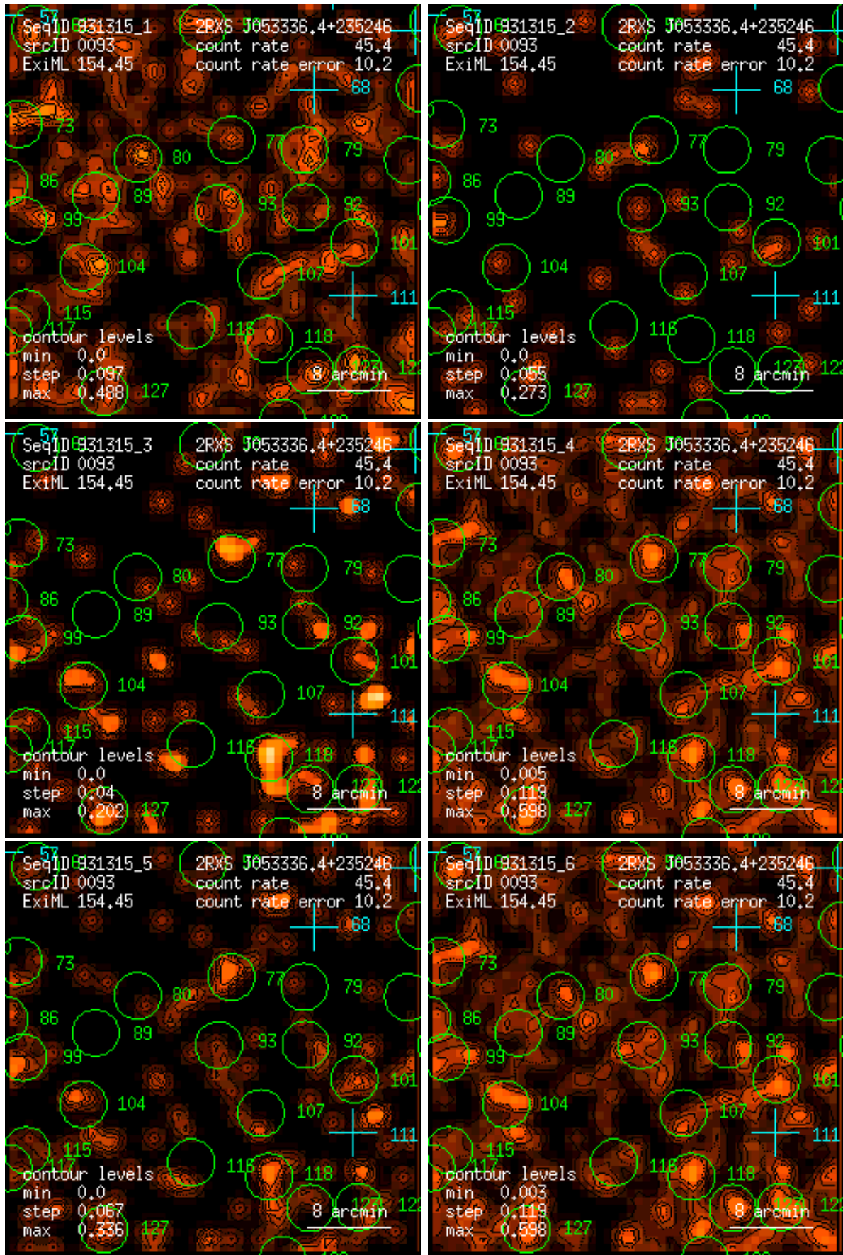
Figure 93: RASS 931315: detection 0093: band rate images, Gaussian filter: (1) PSPC channels 11 – 41, (2) 52 – 90, (3) 91 – 201, (4) 11 – 235, (5) 52 – 201, (6) 11 – 201. Broad band rates in counts/ks. Band rate contour levels in counts/ks/arcmin 2 .
