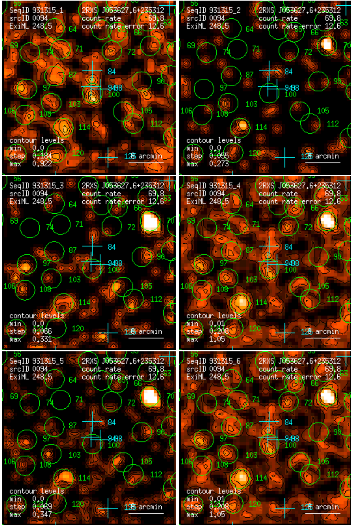
Figure 94: RASS 931315: detection 0094: band rate images, Gaussian filter: (1) PSPC channels 11 – 41, (2) 52 – 90, (3) 91 – 201, (4) 11 – 235, (5) 52 – 201, (6) 11 – 201. Broad band rates in counts/ks. Band rate contour levels in counts/ks/arcmin 2 .
