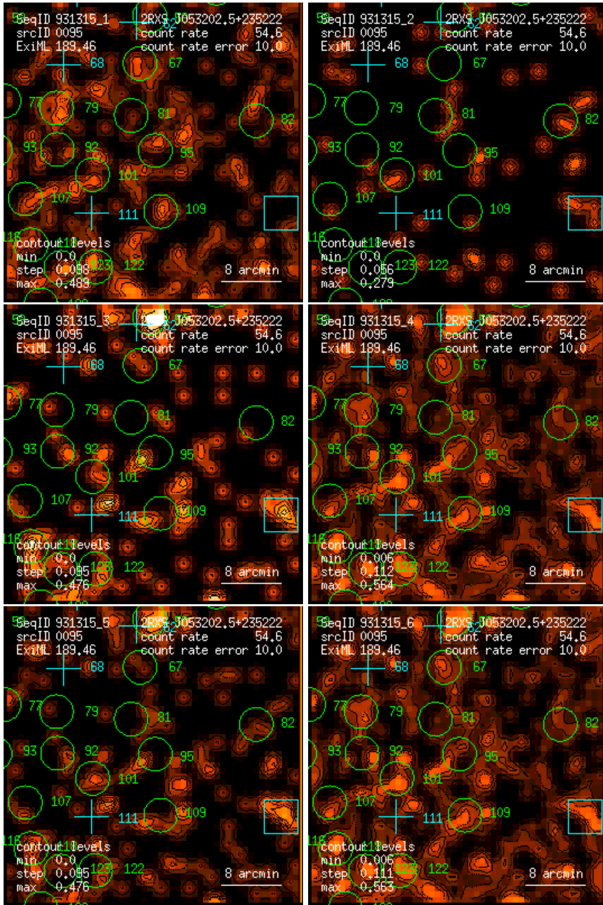
Figure 95: RASS 931315: detection 0095: band rate images, Gaussian filter: (1) PSPC channels 11 – 41, (2) 52 – 90, (3) 91 – 201, (4) 11 – 235, (5) 52 – 201, (6) 11 – 201. Broad band rates in counts/ks. Band rate contour levels in counts/ks/arcmin 2 .
