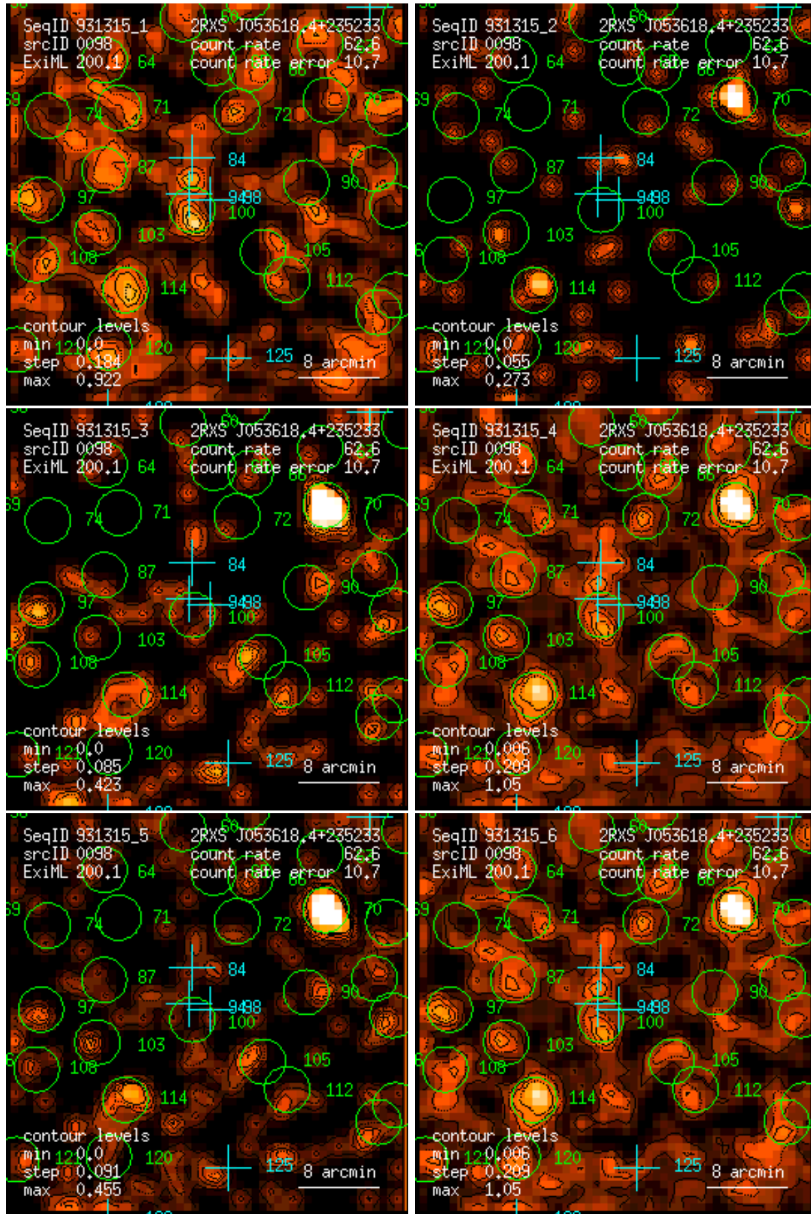
Figure 98: RASS 931315: detection 0098: band rate images, Gaussian filter: (1) PSPC channels 11 – 41, (2) 52 – 90, (3) 91 – 201, (4) 11 – 235, (5) 52 – 201, (6) 11 – 201. Broad band rates in counts/ks. Band rate contour levels in counts/ks/arcmin 2 .
