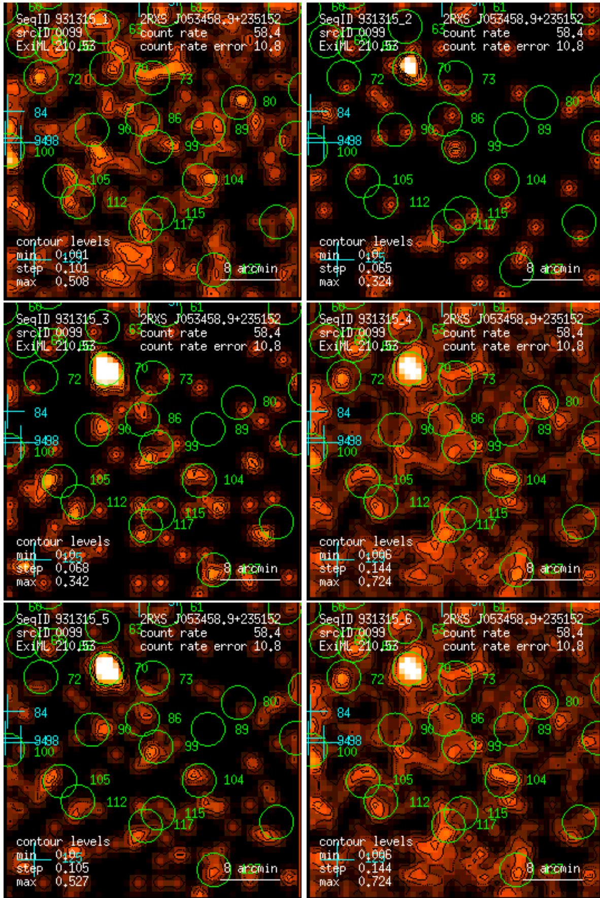
Figure 99: RASS 931315: detection 0099: band rate images, Gaussian filter: (1) PSPC channels 11 – 41, (2) 52 – 90, (3) 91 – 201, (4) 11 – 235, (5) 52 – 201, (6) 11 – 201. Broad band rates in counts/ks. Band rate contour levels in counts/ks/arcmin 2 .
