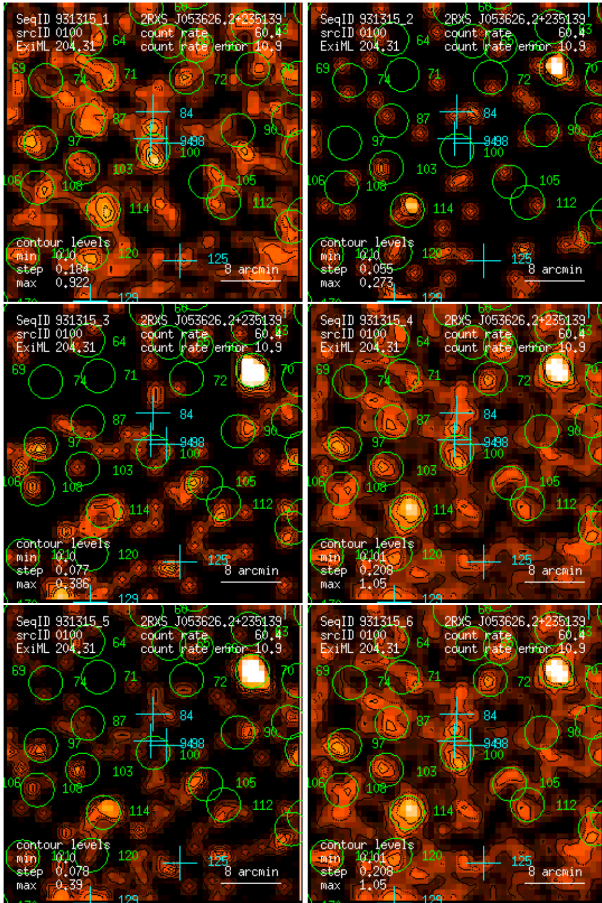
Figure 100: RASS 931315: detection 0100: band rate images, Gaussian filter: (1) PSPC channels 11 – 41, (2) 52 – 90, (3) 91 – 201, (4) 11 – 235, (5) 52 – 201, (6) 11 – 201. Broad band rates in counts/ks. Band rate contour levels in counts/ks/arcmin 2 .
