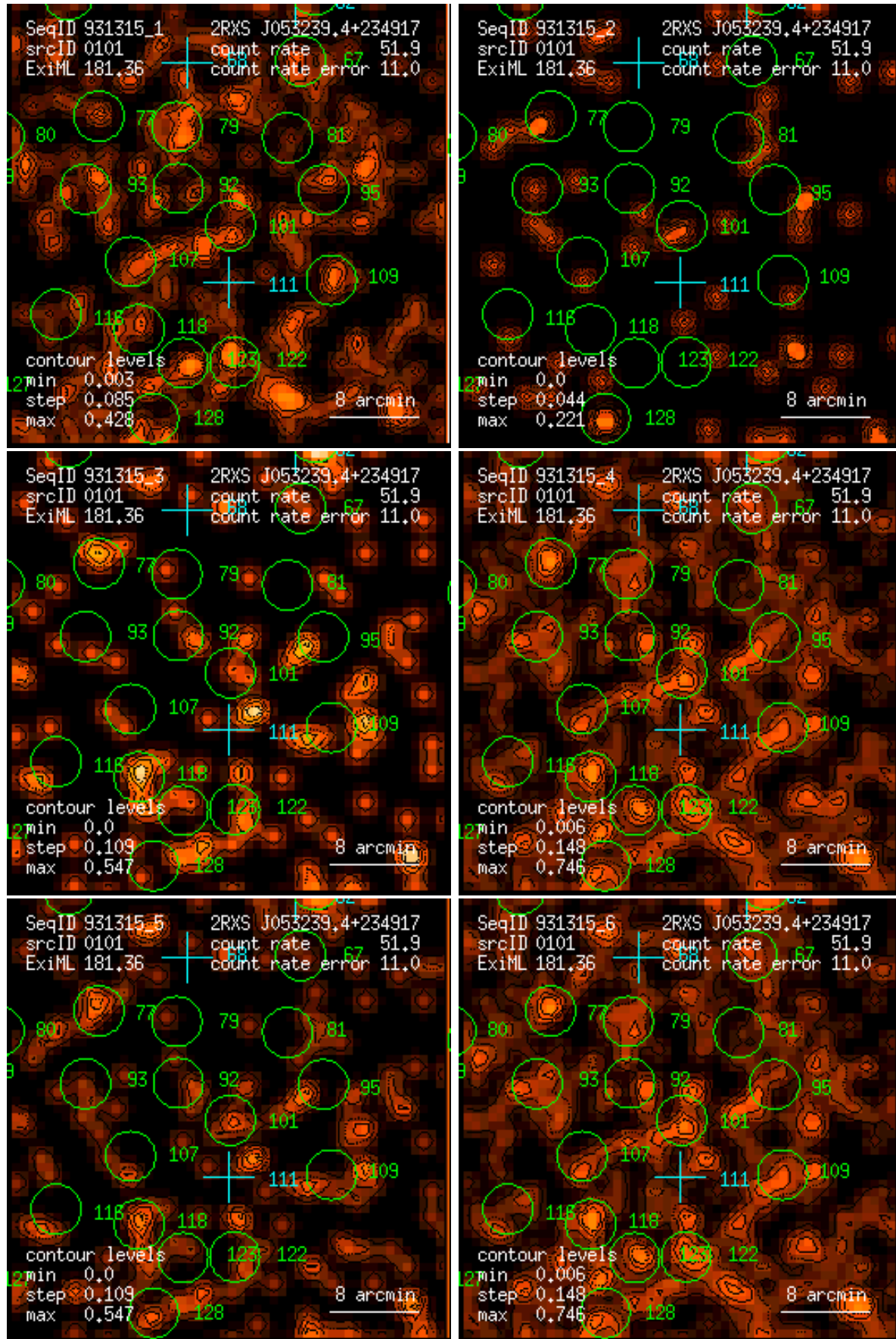
Figure 101: RASS 931315: detection 0101: band rate images, Gaussian filter: (1) PSPC channels 11 – 41, (2) 52 – 90, (3) 91 – 201, (4) 11 – 235, (5) 52 – 201, (6) 11 – 201. Broad band rates in counts/ks. Band rate contour levels in counts/ks/arcmin 2 .
