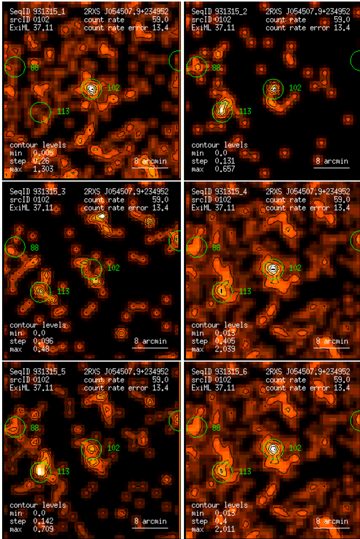
Figure 102: RASS 931315: detection 0102: band rate images, Gaussian filter: (1) PSPC channels 11 – 41, (2) 52 – 90, (3) 91 – 201, (4) 11 – 235, (5) 52 – 201, (6) 11 – 201. Broad band rates in counts/ks. Band rate contour levels in counts/ks/arcmin 2 .
