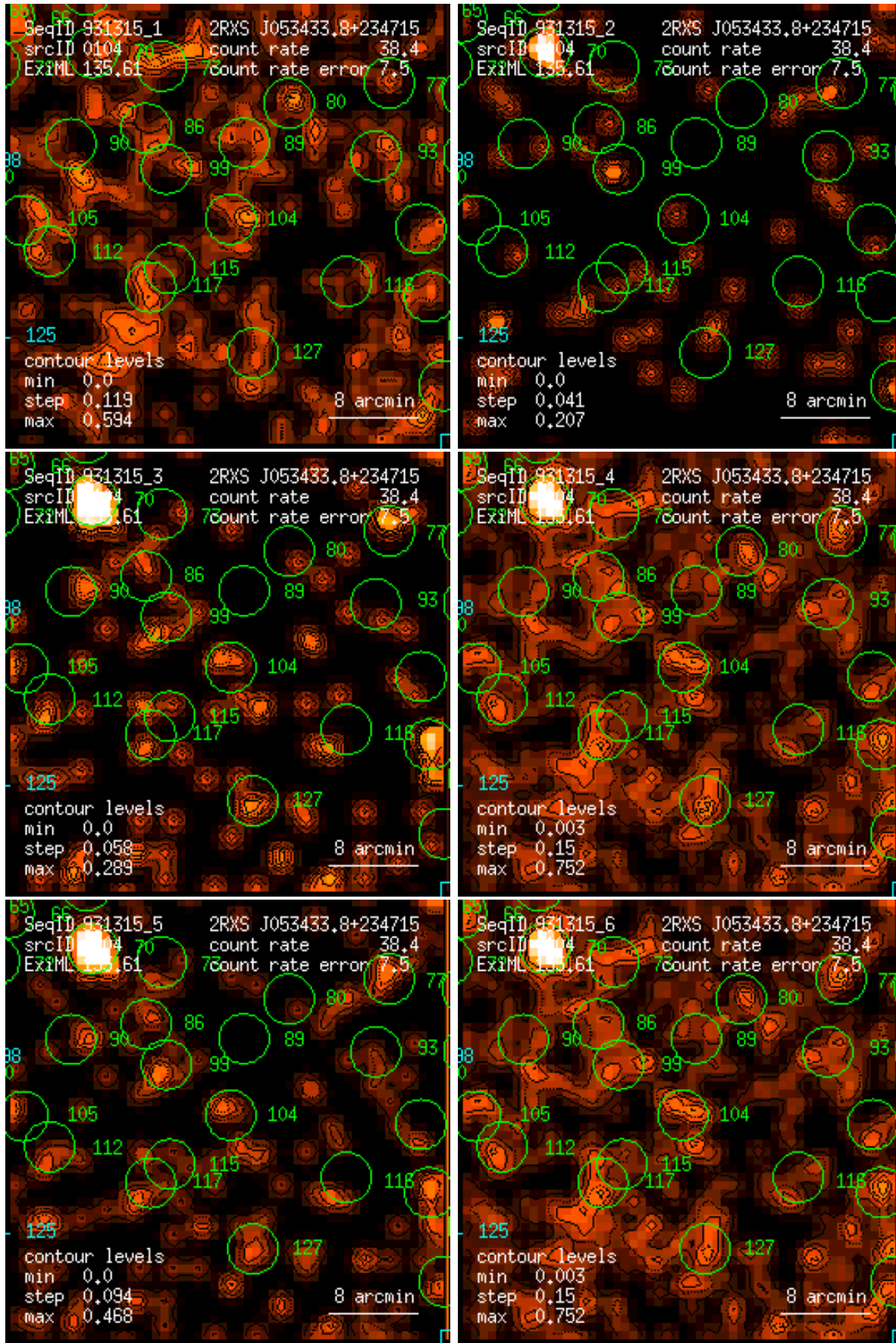
Figure 104: RASS 931315: detection 0104: band rate images, Gaussian filter: (1) PSPC channels 11 – 41, (2) 52 – 90, (3) 91 – 201, (4) 11 – 235, (5) 52 – 201, (6) 11 – 201. Broad band rates in counts/ks. Band rate contour levels in counts/ks/arcmin 2 .
