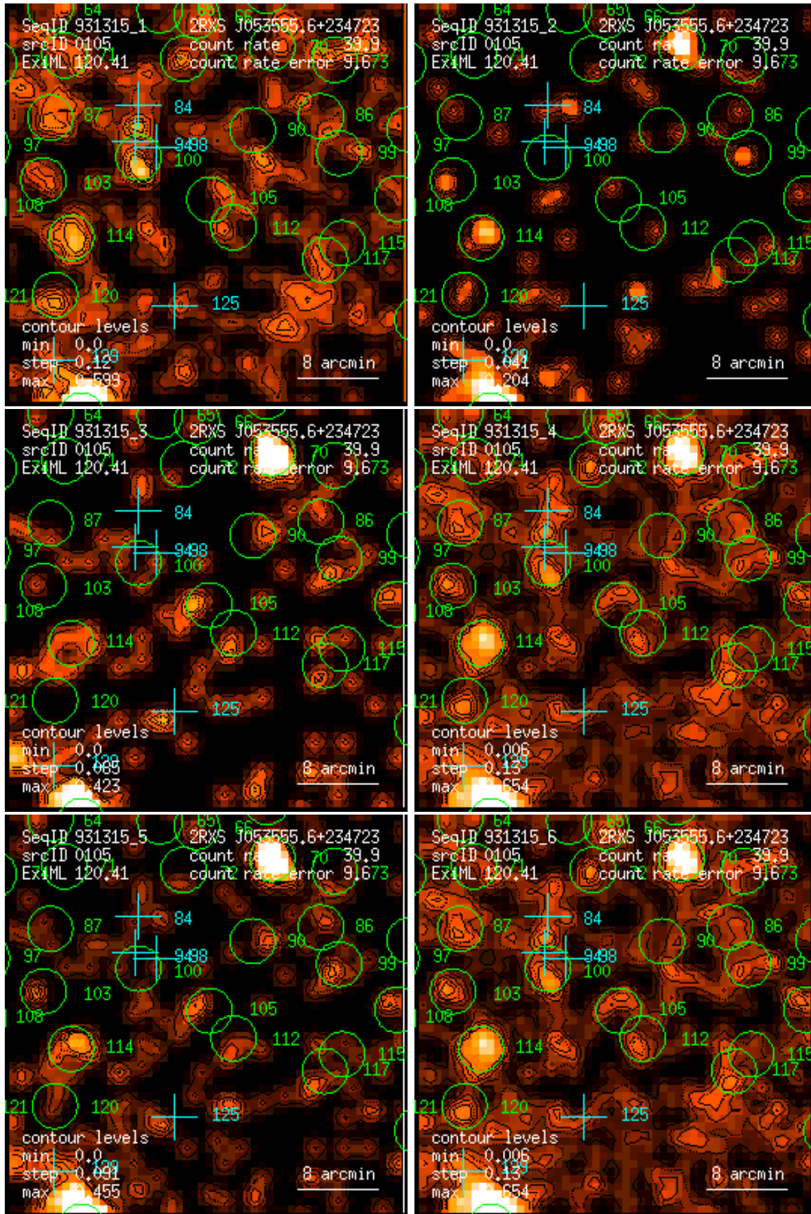
Figure 105: RASS 931315: detection 0105: band rate images, Gaussian filter: (1) PSPC channels 11 – 41, (2) 52 – 90, (3) 91 – 201, (4) 11 – 235, (5) 52 – 201, (6) 11 – 201. Broad band rates in counts/ks. Band rate contour levels in counts/ks/arcmin 2 .
