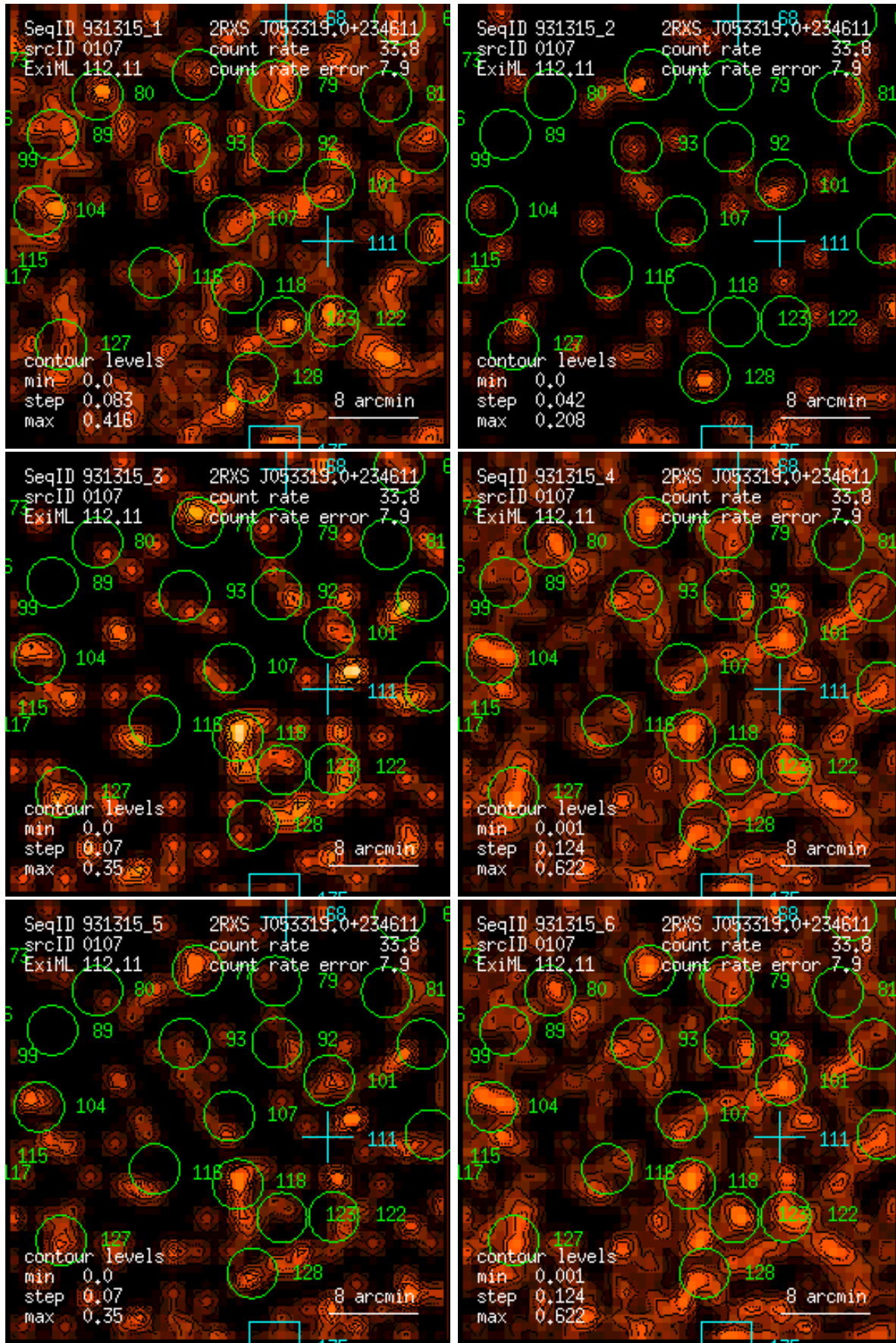
Figure 107: RASS 931315: detection 0107: band rate images, Gaussian filter: (1) PSPC channels 11 – 41, (2) 52 – 90, (3) 91 – 201, (4) 11 – 235, (5) 52 – 201, (6) 11 – 201. Broad band rates in counts/ks. Band rate contour levels in counts/ks/arcmin 2 .
