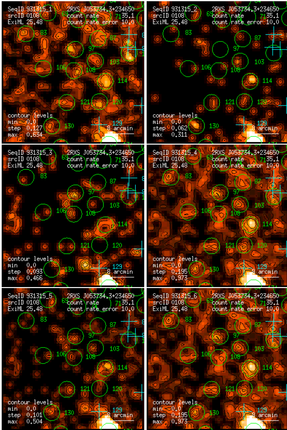
Figure 108: RASS 931315: detection 0108: band rate images, Gaussian filter: (1) PSPC channels 11 – 41, (2) 52 – 90, (3) 91 – 201, (4) 11 – 235, (5) 52 – 201, (6) 11 – 201. Broad band rates in counts/ks. Band rate contour levels in counts/ks/arcmin 2 .
