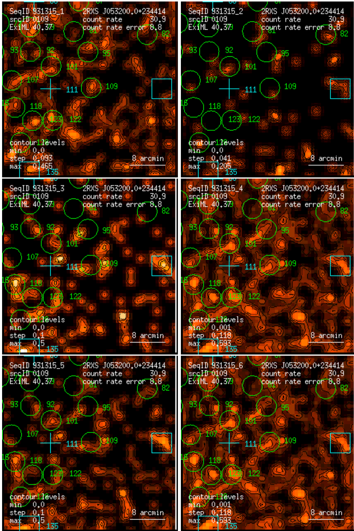
Figure 109: RASS 931315: detection 0109: band rate images, Gaussian filter: (1) PSPC channels 11 – 41, (2) 52 – 90, (3) 91 – 201, (4) 11 – 235, (5) 52 – 201, (6) 11 – 201. Broad band rates in counts/ks. Band rate contour levels in counts/ks/arcmin 2 .
