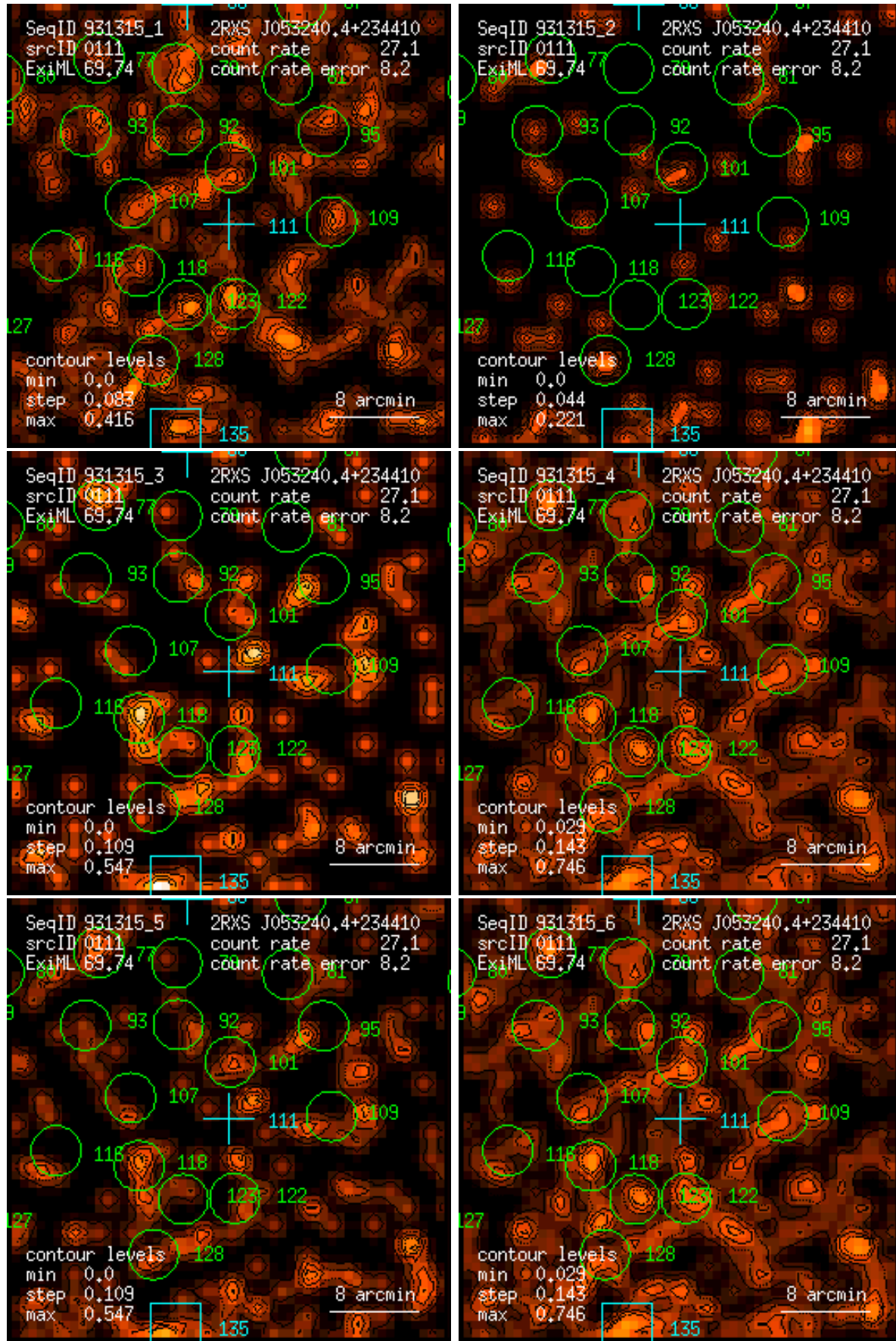
Figure 111: RASS 931315: detection 0111: band rate images, Gaussian filter: (1) PSPC channels 11 – 41, (2) 52 – 90, (3) 91 – 201, (4) 11 – 235, (5) 52 – 201, (6) 11 – 201. Broad band rates in counts/ks. Band rate contour levels in counts/ks/arcmin 2 .
