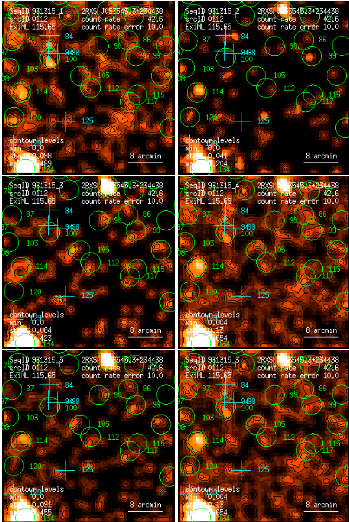
Figure 112: RASS 931315: detection 0112: band rate images, Gaussian filter: (1) PSPC channels 11 – 41, (2) 52 – 90, (3) 91 – 201, (4) 11 – 235, (5) 52 – 201, (6) 11 – 201. Broad band rates in counts/ks. Band rate contour levels in counts/ks/arcmin 2 .
