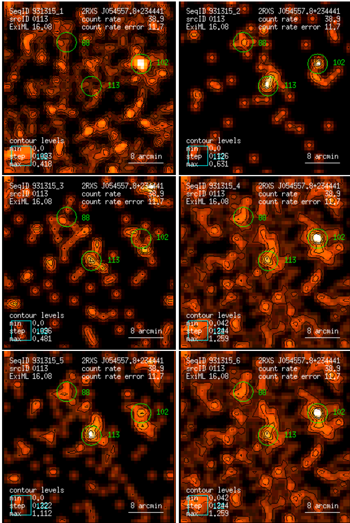
Figure 113: RASS 931315: detection 0113: band rate images, Gaussian filter: (1) PSPC channels 11 – 41, (2) 52 – 90, (3) 91 – 201, (4) 11 – 235, (5) 52 – 201, (6) 11 – 201. Broad band rates in counts/ks. Band rate contour levels in counts/ks/arcmin 2 .
