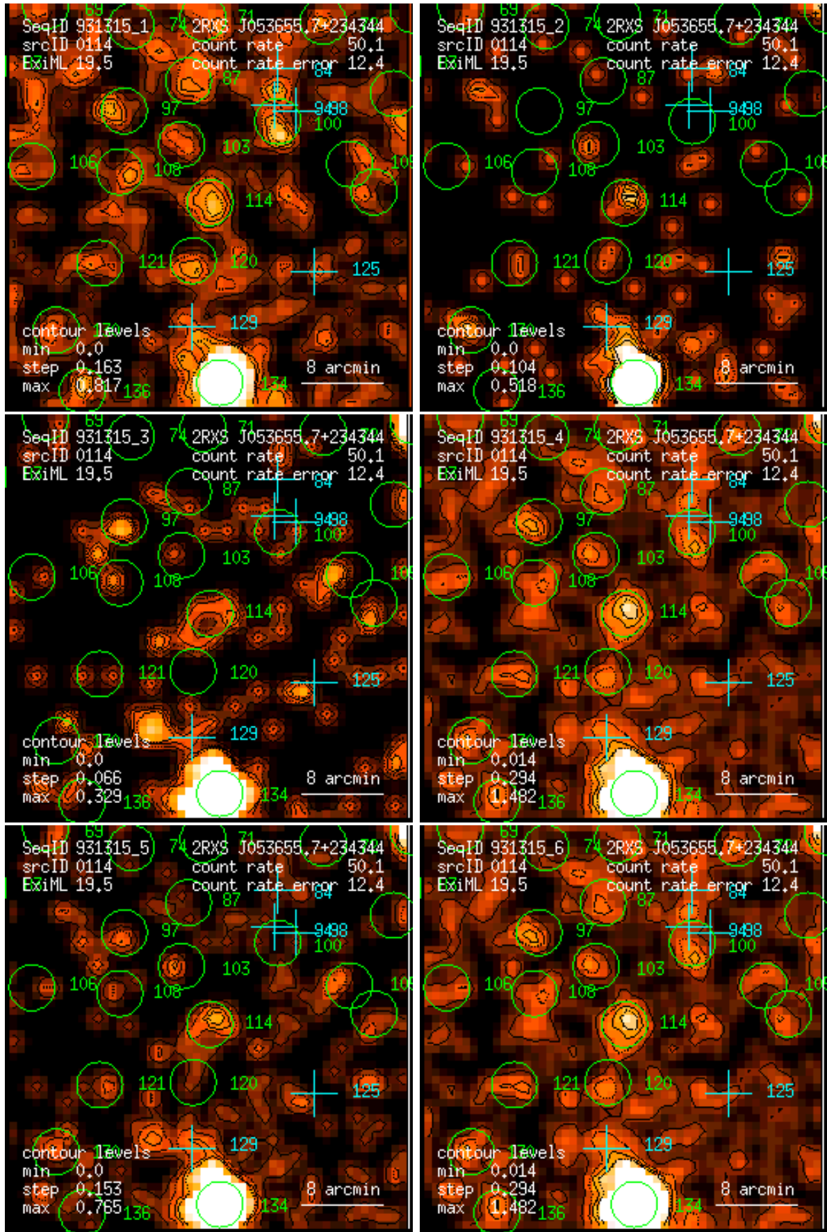
Figure 114: RASS 931315: detection 0114: band rate images, Gaussian filter: (1) PSPC channels 11 – 41, (2) 52 – 90, (3) 91 – 201, (4) 11 – 235, (5) 52 – 201, (6) 11 – 201. Broad band rates in counts/ks. Band rate contour levels in counts/ks/arcmin 2 .
