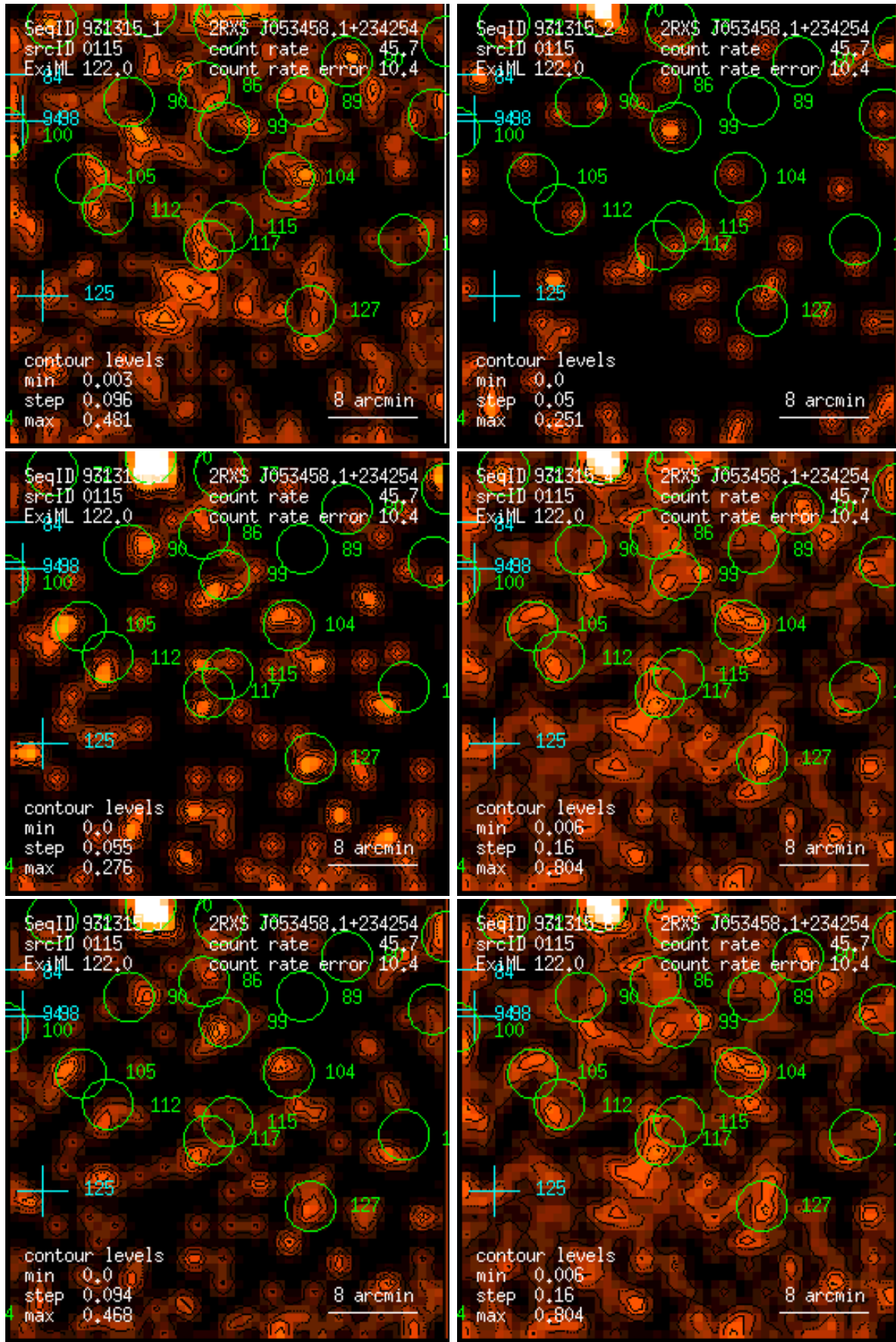
Figure 115: RASS 931315: detection 0115: band rate images, Gaussian filter: (1) PSPC channels 11 – 41, (2) 52 – 90, (3) 91 – 201, (4) 11 – 235, (5) 52 – 201, (6) 11 – 201. Broad band rates in counts/ks. Band rate contour levels in counts/ks/arcmin 2 .
