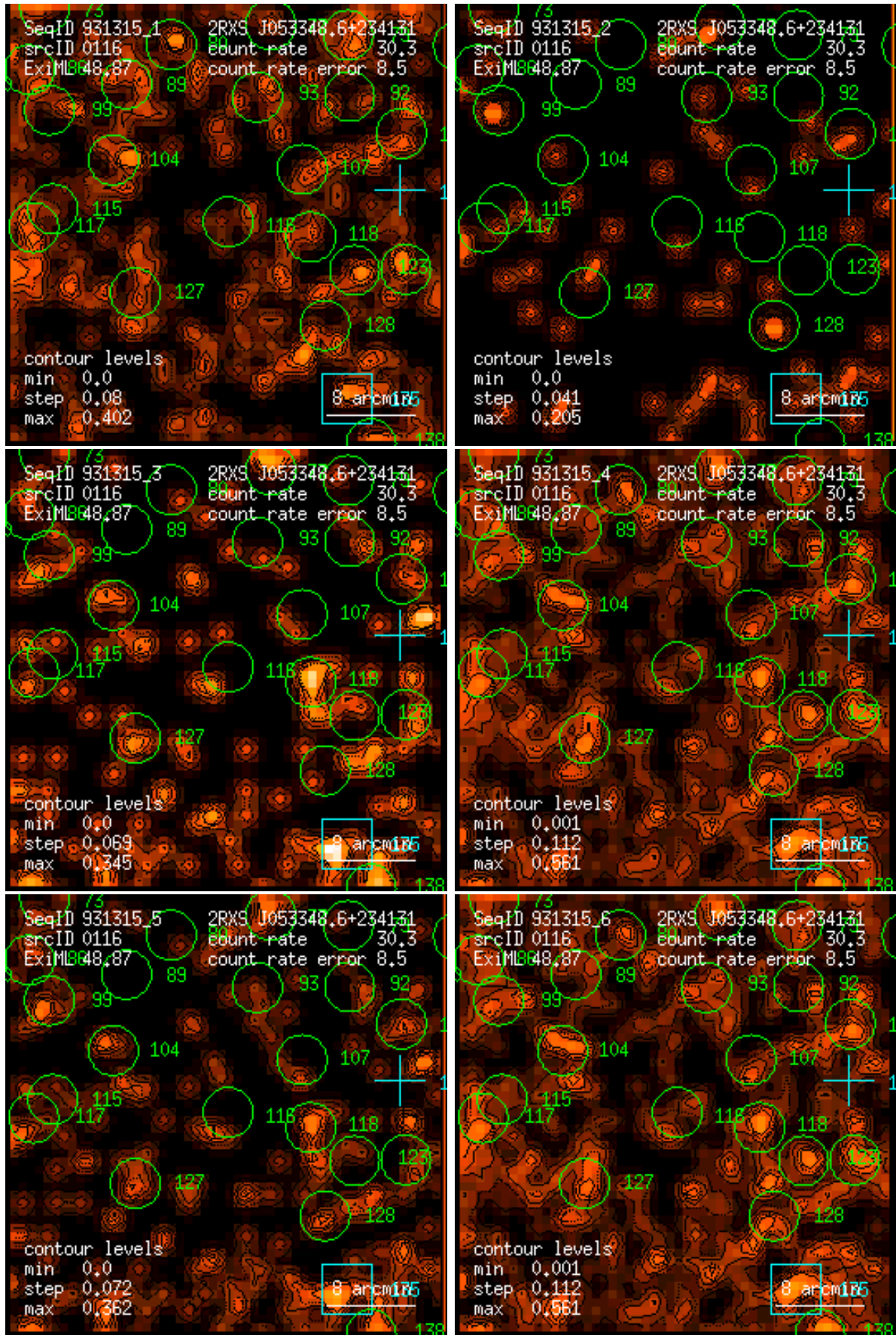
Figure 116: RASS 931315: detection 0116: band rate images, Gaussian filter: (1) PSPC channels 11 – 41, (2) 52 – 90, (3) 91 – 201, (4) 11 – 235, (5) 52 – 201, (6) 11 – 201. Broad band rates in counts/ks. Band rate contour levels in counts/ks/arcmin 2 .
