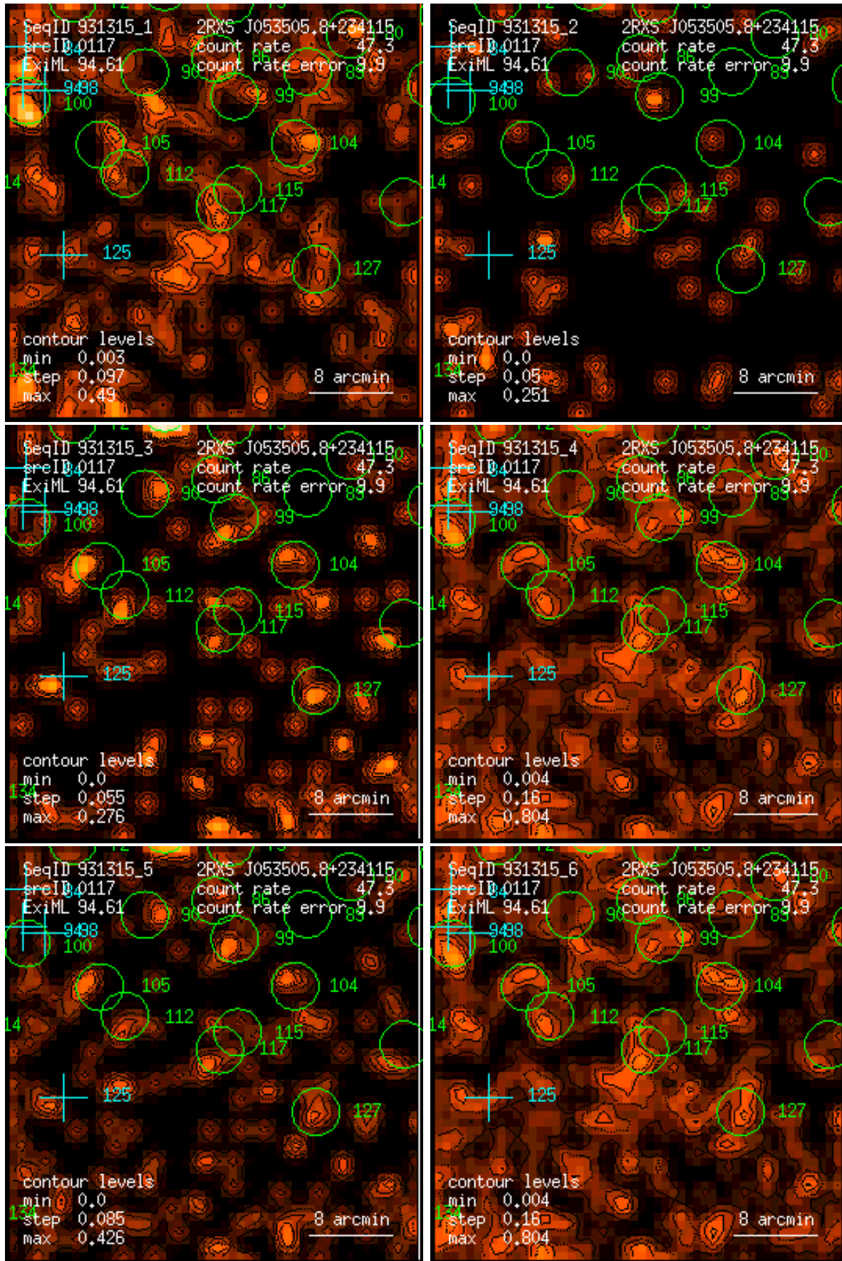
Figure 117: RASS 931315: detection 0117: band rate images, Gaussian filter: (1) PSPC channels 11 – 41, (2) 52 – 90, (3) 91 – 201, (4) 11 – 235, (5) 52 – 201, (6) 11 – 201. Broad band rates in counts/ks. Band rate contour levels in counts/ks/arcmin 2 .
