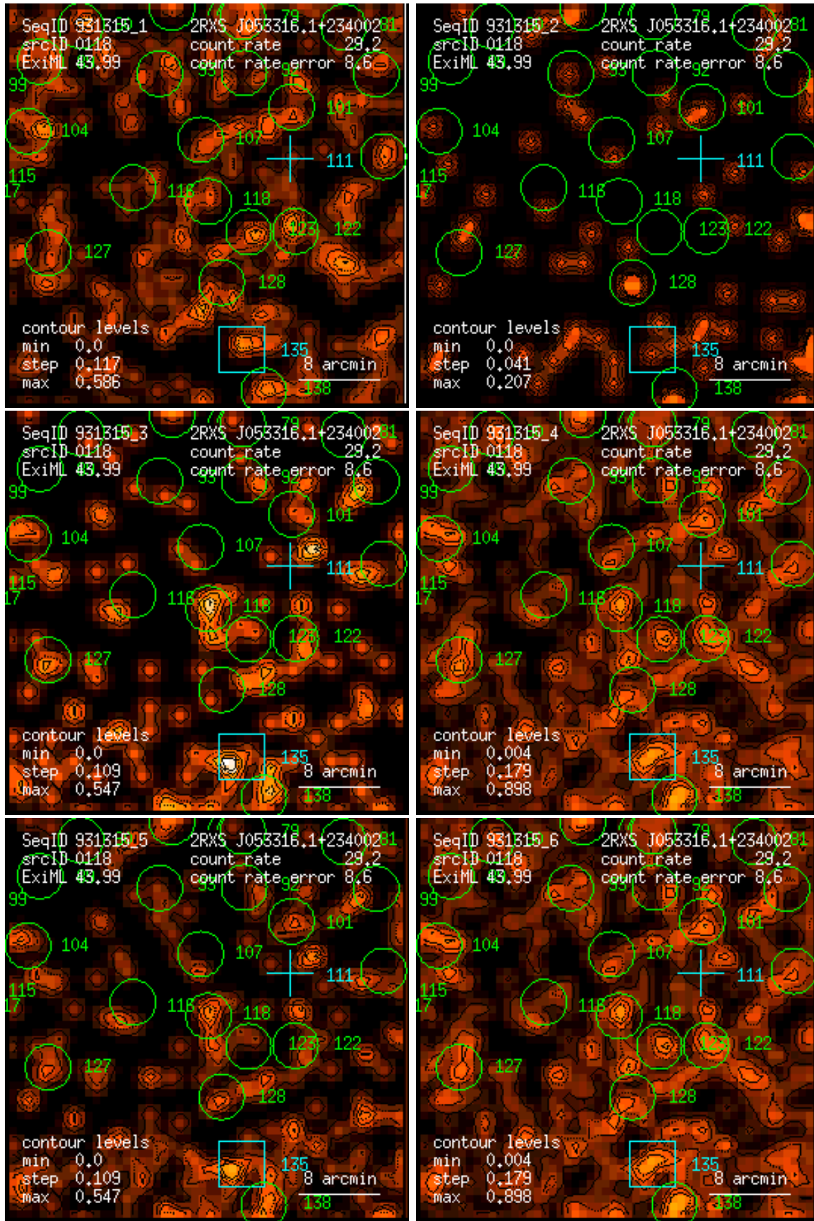
Figure 118: RASS 931315: detection 0118: band rate images, Gaussian filter: (1) PSPC channels 11 – 41, (2) 52 – 90, (3) 91 – 201, (4) 11 – 235, (5) 52 – 201, (6) 11 – 201. Broad band rates in counts/ks. Band rate contour levels in counts/ks/arcmin 2 .
