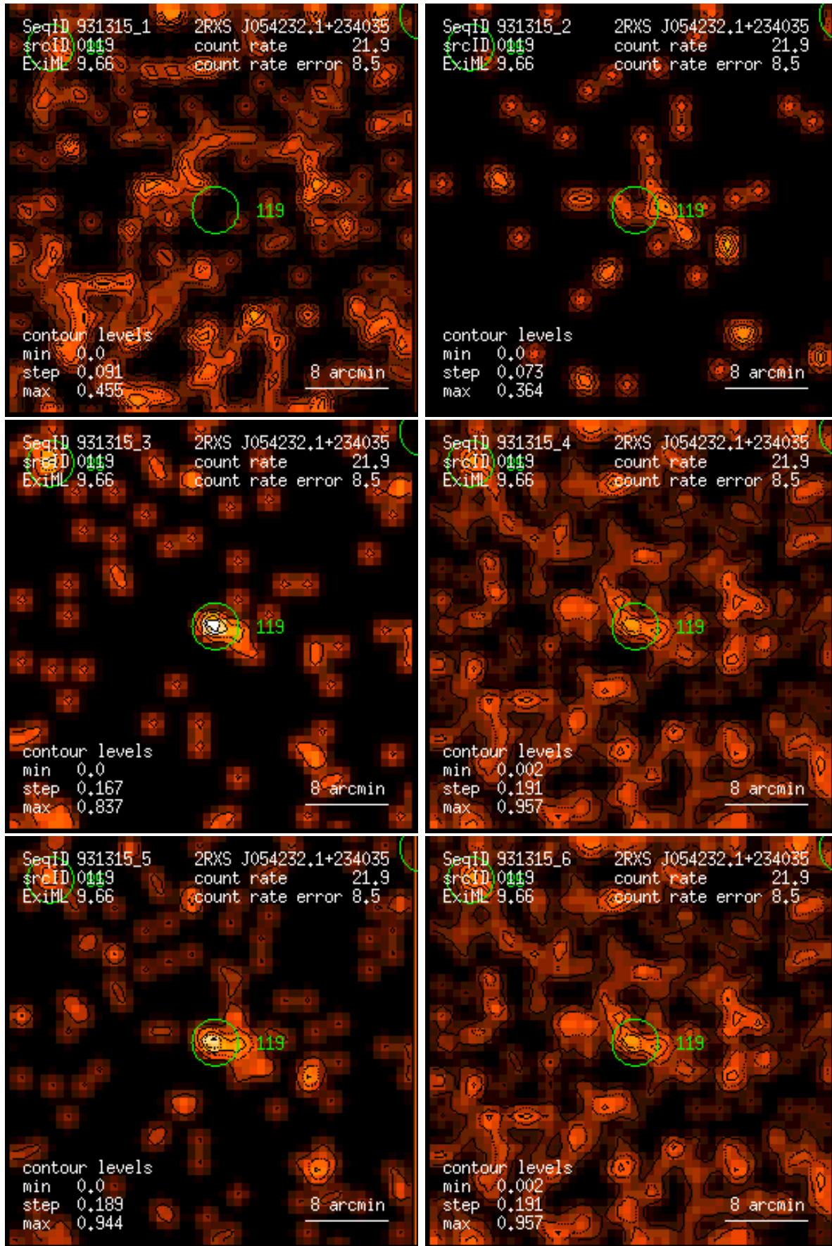
Figure 119: RASS 931315: detection 0119: band rate images, Gaussian filter: (1) PSPC channels 11 – 41, (2) 52 – 90, (3) 91 – 201, (4) 11 – 235, (5) 52 – 201, (6) 11 – 201. Broad band rates in counts/ks. Band rate contour levels in counts/ks/arcmin 2 .
