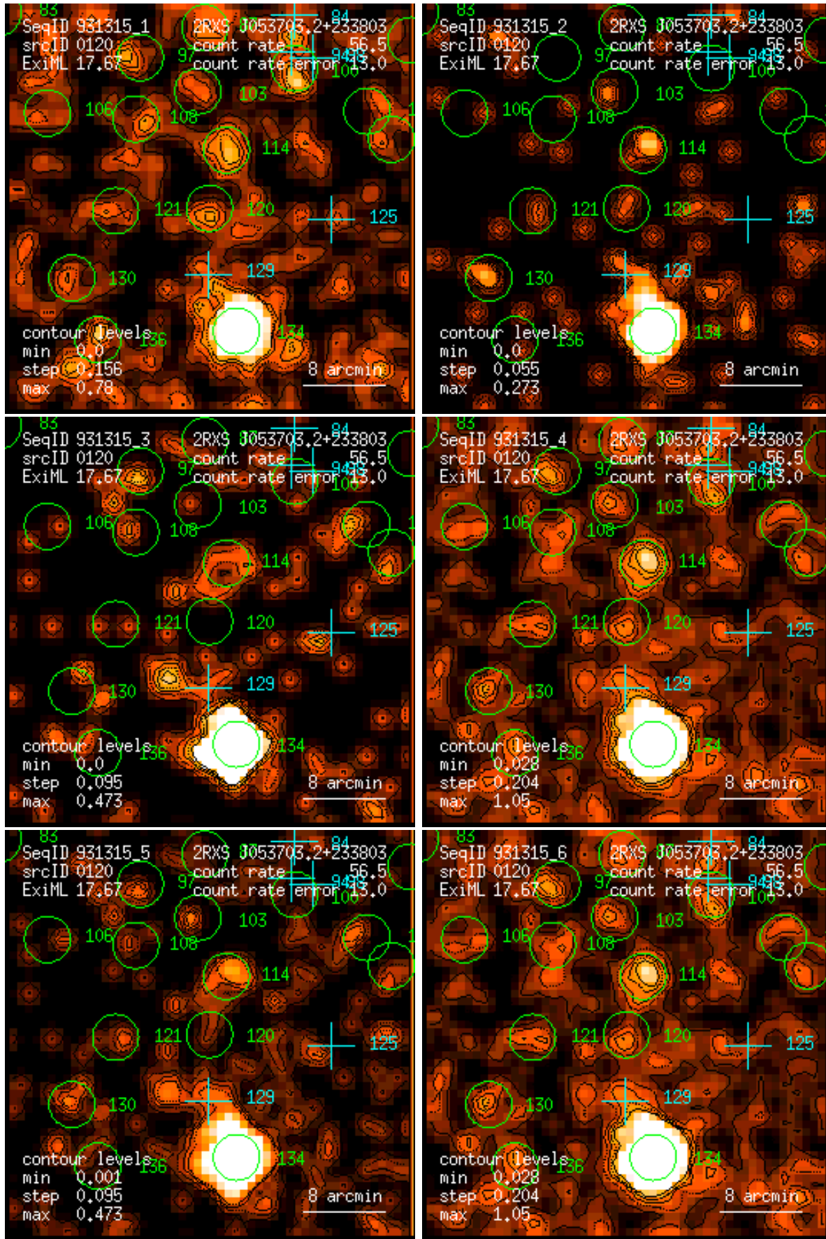
Figure 120: RASS 931315: detection 0120: band rate images, Gaussian filter: (1) PSPC channels 11 – 41, (2) 52 – 90, (3) 91 – 201, (4) 11 – 235, (5) 52 – 201, (6) 11 – 201. Broad band rates in counts/ks. Band rate contour levels in counts/ks/arcmin 2 .
