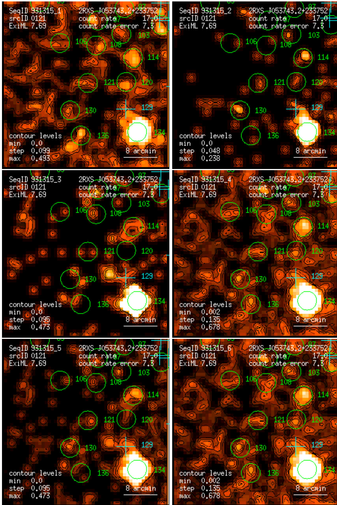
Figure 121: RASS 931315: detection 0121: band rate images, Gaussian filter: (1) PSPC channels 11 – 41, (2) 52 – 90, (3) 91 – 201, (4) 11 – 235, (5) 52 – 201, (6) 11 – 201. Broad band rates in counts/ks. Band rate contour levels in counts/ks/arcmin 2 .
