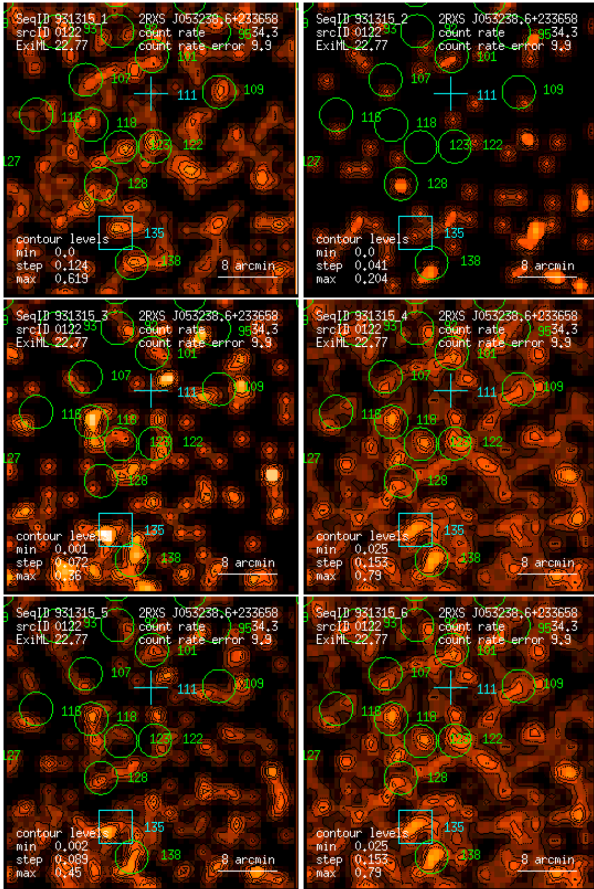
Figure 122: RASS 931315: detection 0122: band rate images, Gaussian filter: (1) PSPC channels 11 – 41, (2) 52 – 90, (3) 91 – 201, (4) 11 – 235, (5) 52 – 201, (6) 11 – 201. Broad band rates in counts/ks. Band rate contour levels in counts/ks/arcmin 2 .
