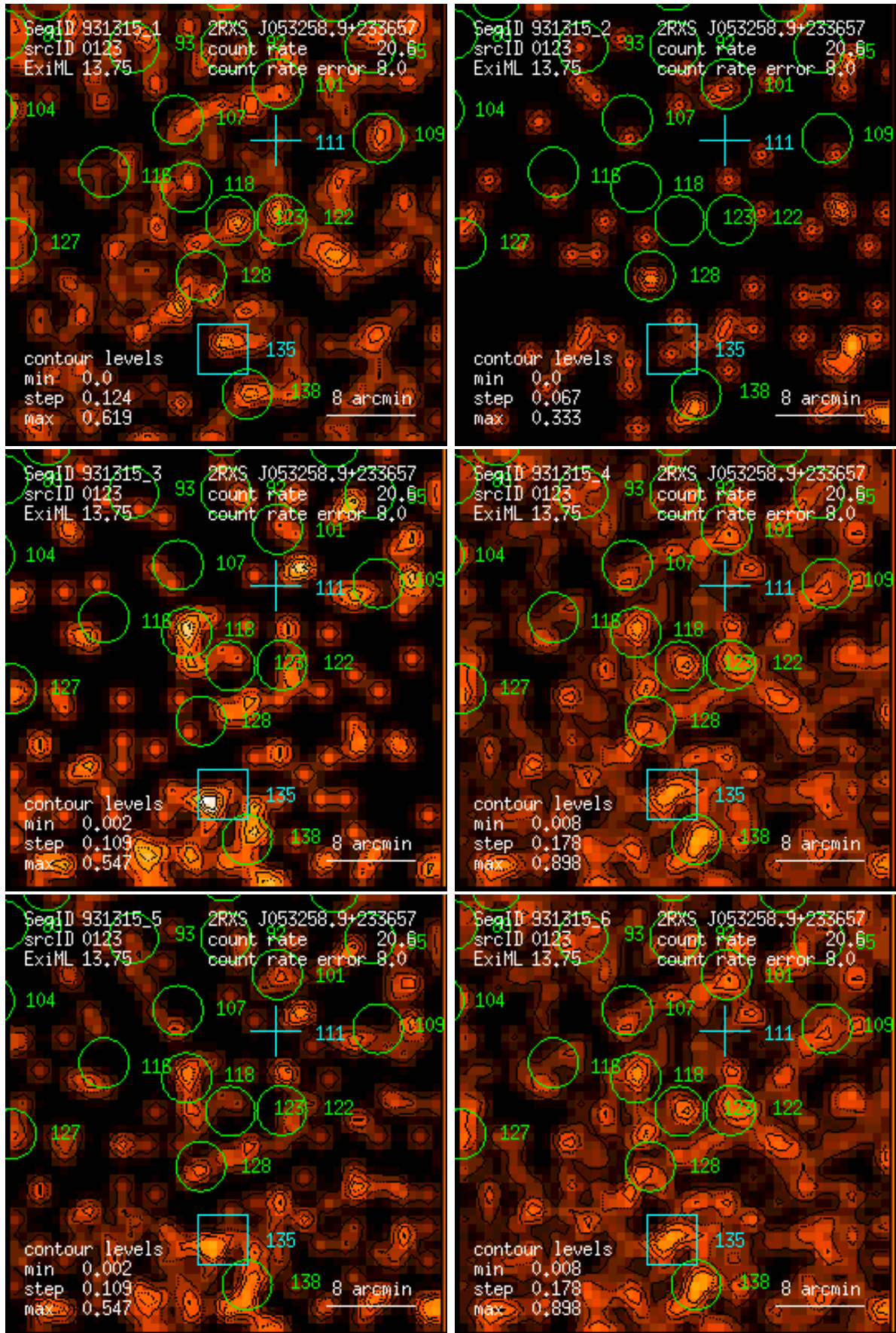
Figure 123: RASS 931315: detection 0123: band rate images, Gaussian filter: (1) PSPC channels 11 – 41, (2) 52 – 90, (3) 91 – 201, (4) 11 – 235, (5) 52 – 201, (6) 11 – 201. Broad band rates in counts/ks. Band rate contour levels in counts/ks/arcmin 2 .
