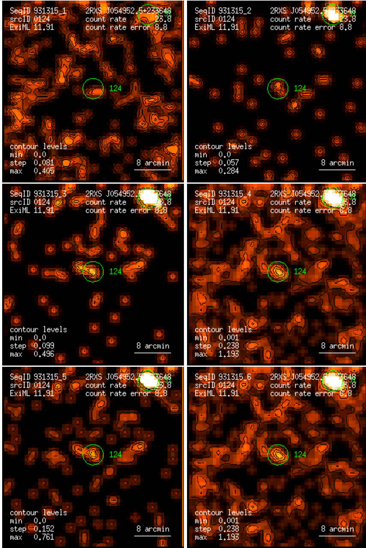
Figure 124: RASS 931315: detection 0124: band rate images, Gaussian filter: (1) PSPC channels 11 – 41, (2) 52 – 90, (3) 91 – 201, (4) 11 – 235, (5) 52 – 201, (6) 11 – 201. Broad band rates in counts/ks. Band rate contour levels in counts/ks/arcmin 2 .
