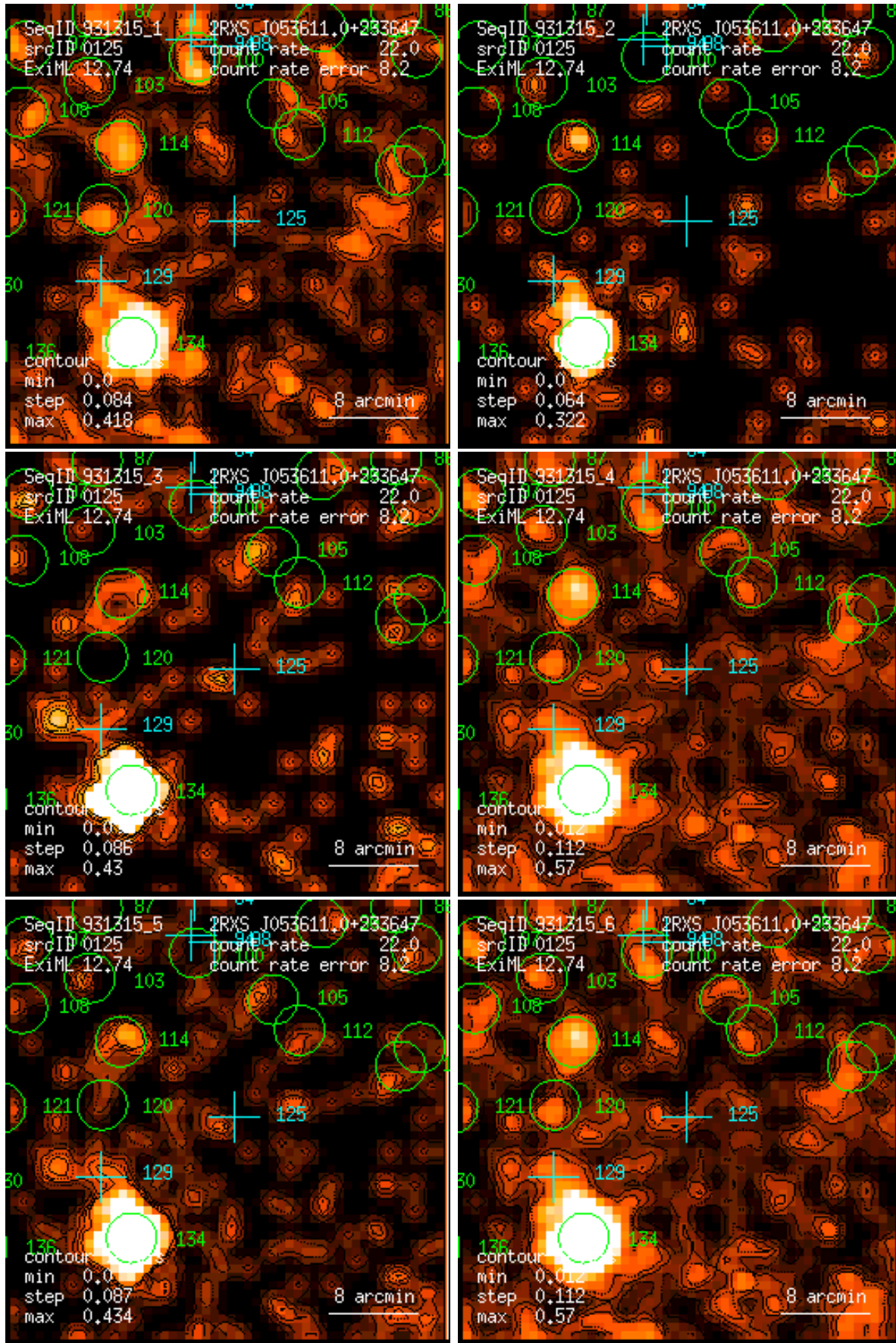
Figure 125: RASS 931315: detection 0125: band rate images, Gaussian filter: (1) PSPC channels 11 – 41, (2) 52 – 90, (3) 91 – 201, (4) 11 – 235, (5) 52 – 201, (6) 11 – 201. Broad band rates in counts/ks. Band rate contour levels in counts/ks/arcmin 2 .
