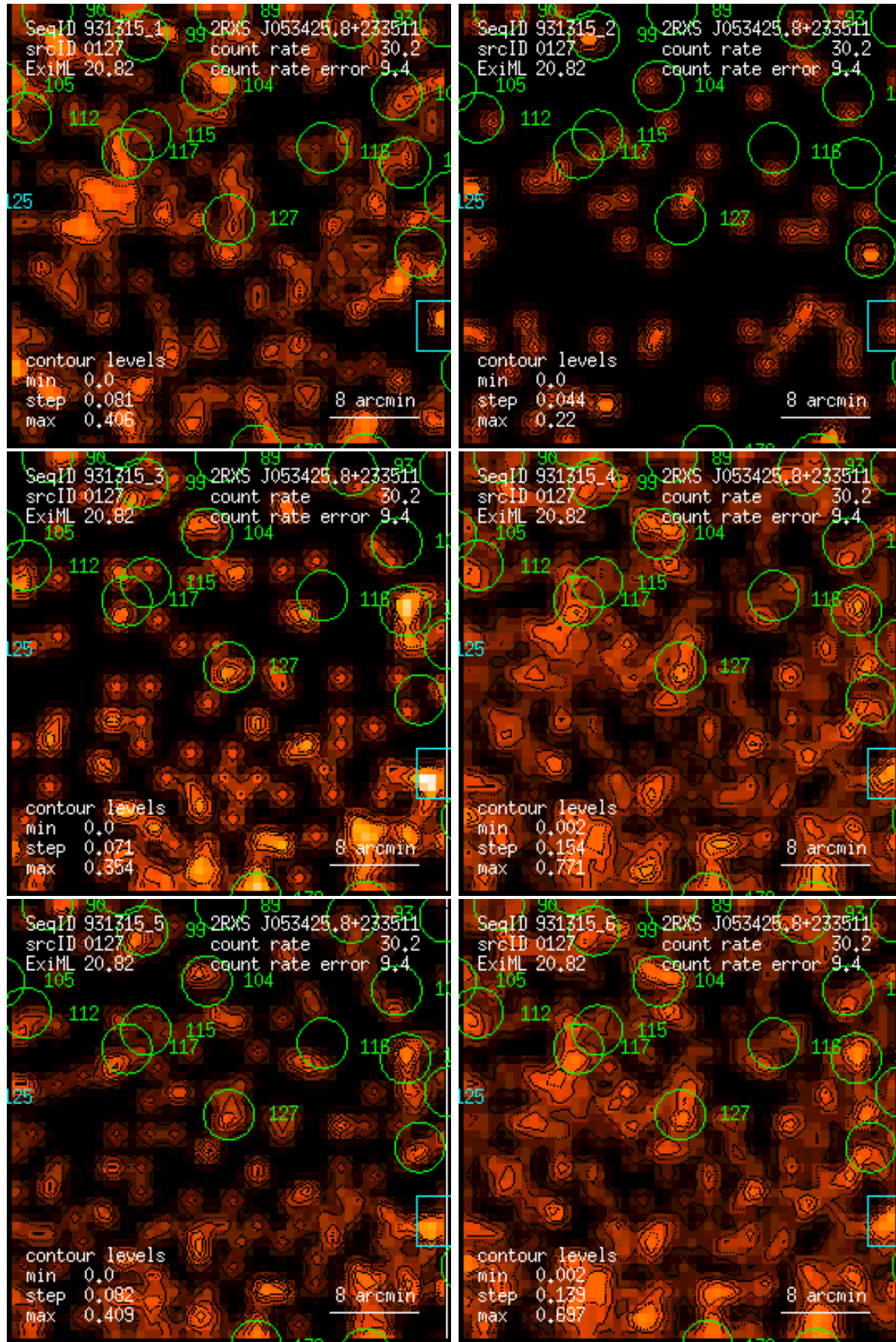
Figure 127: RASS 931315: detection 0127: band rate images, Gaussian filter: (1) PSPC channels 11 – 41, (2) 52 – 90, (3) 91 – 201, (4) 11 – 235, (5) 52 – 201, (6) 11 – 201. Broad band rates in counts/ks. Band rate contour levels in counts/ks/arcmin 2 .
